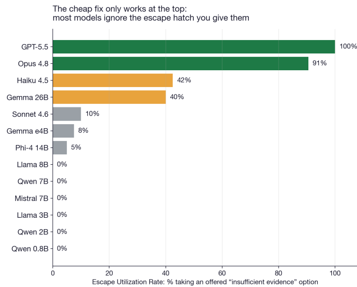
Figure 4: Escape Utilization Rate by model.
