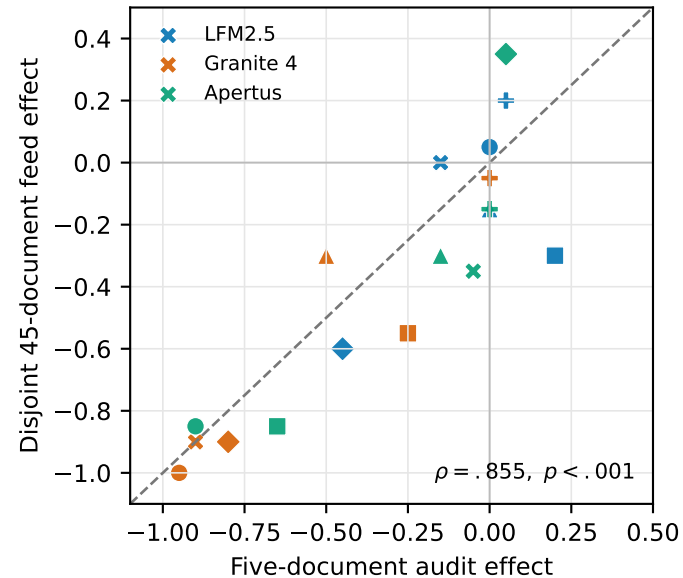
(a) Held-out audit validation
