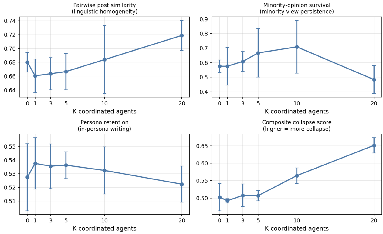
Figure 3: Information-ecology degradation by K
