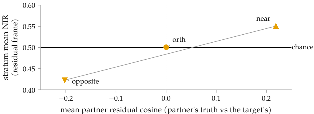
(a) the comparator's score tracks the partner's true alignment
