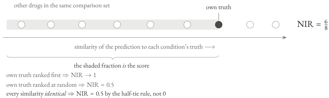
FIGURE 4.2 NIR asks whether a prediction resembles its own condition’s truth more than it resembles the truths of the other conditions in the comparison set J . Own truth ranked first gives \text{NIR} \rightarrow 1 ; ranked at random gives 0.5; and a predictor whose similarities are all identical — the zero vector, which is what “predict the average drug response” becomes in residual space — scores 0.5 by the half-tie rule, not 0.
