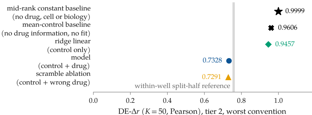
(a) less information, higher score
