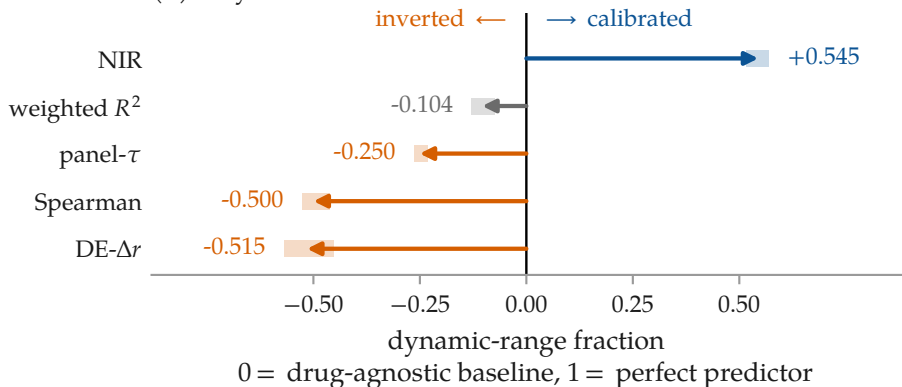
(b) only one metric is calibrated
