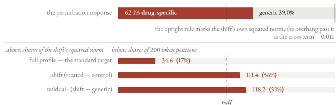
FIGURE 4.15 The drug is the majority of the perturbation response and almost none of the standard target's tokens.
