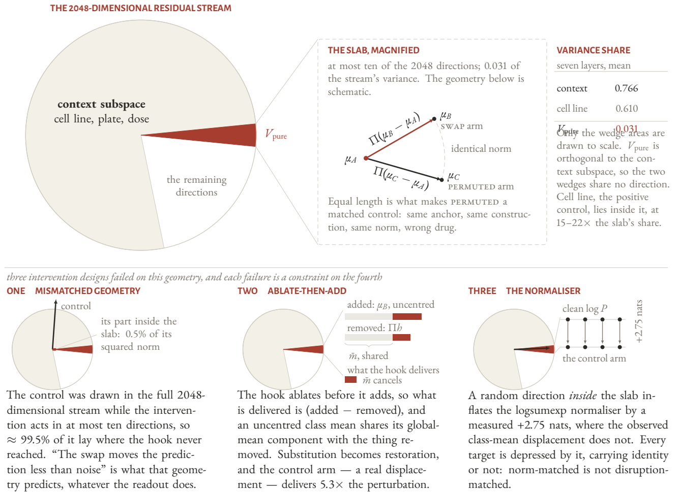
FIGURE A.2 The purified drug slab is a thin wedge of the residual stream beside the context subspace, and each of the three failed identity tests turns on that geometry. The disc is the 2048-dimensional residual stream at one layer. The two wedge areas are the only scaled marks in the figure, drawn to the measured subspace variance shares in workspace_probe.json (twelve drug classes, forty cells each, chance 0.083), averaged over the seven probed layers: 0.766 for the context subspace of cell line, plate and dose, and 0.031 for the purified drug slab V_{\text{pure}} . Cell line alone, the positive control, reads 0.610 and lies inside the context subspace, so it is quoted as a number rather than drawn as a third wedge. V_{\text{pure}} is what remains after the drug slab — spanned by at most eleven directions, since it is built from twelve centred class means, of which the top ten are kept — is orthogonalised against that context subspace, which is why the two wedges share no direction. The unshaded remainder closes the disc and carries no number. Everything else is schematic and has no scale: the slab is 11.3^\circ wide and cannot hold three class means at true size, so its interior is magnified, where the SWAP and PERMUTED displacements are drawn at equal length because equal length is what makes PERMUTED a matched control. The one exception among the insets is inset one's angle, which is drawn true: a direction drawn isotropically in 2048 dimensions puts, on average, 10/2048 of its squared norm in a ten-dimensional slab, the appendix's \approx 99.5\% lying outside it. No decode accuracy, layer axis or KL divergence appears here; those are Figure 4.7. The three insets are the failed designs of § A.5.
