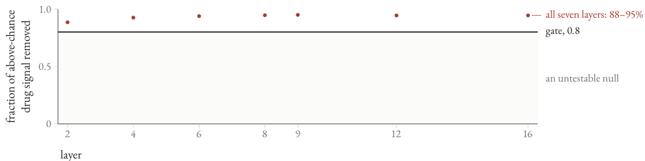
FIGURE 4.8 The slab is built, not found — ten directions fitted to twelve centred class means, then orthogonalised against the batch structure they are confounded with — and the raw slab earns the right to be purified and ablated only because projecting it out destroys 88 to 95 per cent of the decodable drug signal at every depth. (a) Where the twelve drug classes differ at one depth, giving V_{\text{drug}} . (b) Why the raw slab may not be used: it is partly a batch subspace, and the darker patch on the band is the component projected away to leave V_{\text{pure}} , on which every causal claim in this chapter is made. Neither panel has a scale — nothing in them is a measurement, and the four printed numbers are the only sourced quantities there. (c) The removal gate, and the only panel with a scale: each mark is one depth's share of above-chance drug-label accuracy destroyed when the subspace is projected out, over twelve classes at chance 1/12. The shaded region below the rule is the set of outcomes that would have left every null in this section untestable, and it is empty at all seven depths. No interval is drawn: the quantity is a single ratio of two accuracies over 480 prompts, with no stored dispersion. These twelve-class accuracies must not be read against the twenty-four-class sweep of § 4.5, whose chance is 1/24.
