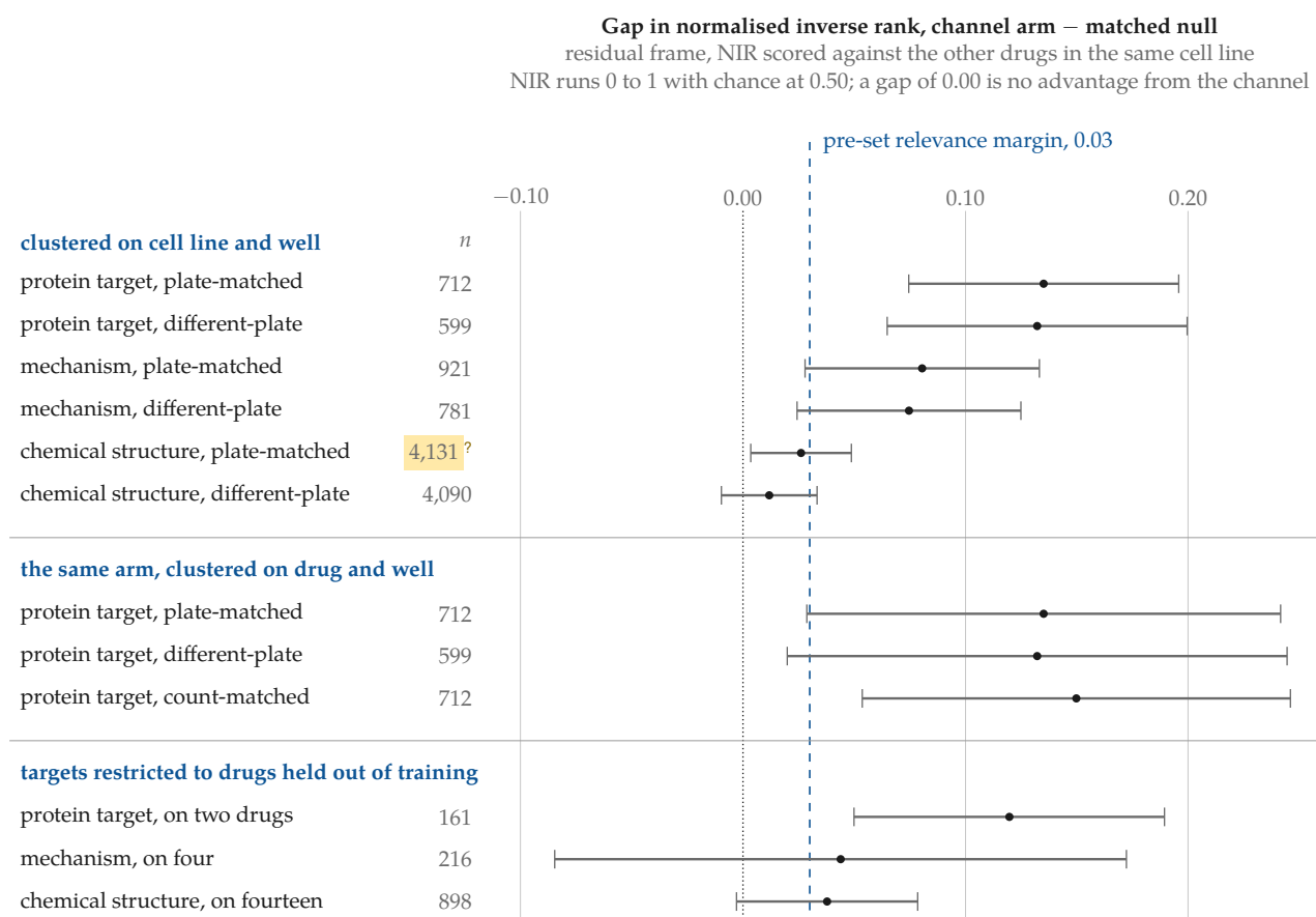
Figure 4.21. The gate's verdict is decided by what the interval is conditioned on, not by where the point estimate falls. Every row is residual-frame NIR scored against the other drugs in the same cell line: the arm predicts a drug's residual from its annotated neighbours there, and its matched null draws the same number of partner drugs from that cell line. The dot is the estimate, the bar its 95% two-way cluster-robust interval, the dashed line the pre-set relevance margin of 0.03 that the gate asks the lower bound to clear. The count beside each row label is the number of conditions that row scores, not of drugs; the first block's plate-matched counts are the n of Table 4.13. The second block re-clusters the same target arm on the drug, the unit a claim about unseen drugs has to generalise across, leaving the point estimates untouched; the lower bound now falls short against both estimand-correct nulls and only the weaker count-matched one clears it. The third restricts the targets to drugs held out of training. Rows may be read within a block and not across blocks.
