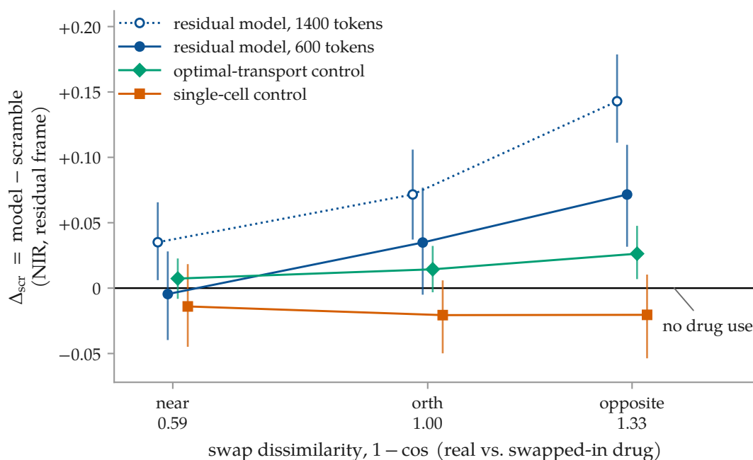
Figure 4.17. On the earlier target build, the residual model’s advantage over its own scramble grew with how dissimilar the swapped-in drug’s residual was; the single-cell control scored through the identical pipeline stayed flat and null, while the optimal-transport control did not. Residual frame throughout. The horizontal axis is measured swap dissimilarity, 1 - \cos between the real and the swapped-in drug’s residual, byte-identical across all four runs, so the three stratum positions are exact; the connecting lines are guides between three measured strata and not a sampled continuum, and the four series are nudged sideways so that their intervals do not overlap. The three solid series are at a matched 600-token budget; the residual model’s 1400-token run is the dotted overlay, since the budget alone roughly doubles the gap on the two strata where it is positive at 600 ( +0.0349 \rightarrow +0.0716 on orth, +0.0716 \rightarrow +0.1429 on opposite). Intervals are 95% bootstrap clustered over cell lines, n = 250 conditions per point. The near stratum is the weakest test by construction, since where the swapped-in drug’s true residual is similar, an unchanged prediction is correct.
