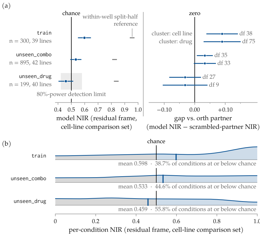
Figure 4.18. The residual-frame model clears chance on trained conditions only; the held-out-combination gap excludes zero clustered on cell line but not clustered on drug, and the unseen-drug gap flips sign. Residual frame throughout, and NIR ranks each prediction against the other drugs measured in the same cell line. (a) Left, model NIR against the chance value 0.5 (solid rule), with 95% two-way cluster-robust intervals; n = 300, 895 and 199 conditions on train, unseen_combo and unseen_drug. The grey dash on each row is that split's raw within-well split-half precision reference, a measurement-precision figure computed from two halves of the same well and not a replicate experiment; it carries no interval and is drawn as a bare marker, and only train is filtered at the reliability line. Right, on its own axis, the gap against the geometry-defined orth partner. Each row has one point estimate, drawn twice with two intervals because the verdict depends on which unit of generalisation is clustered: cell-line-clustered above, drug-clustered below, each labelled with the Student t degrees of freedom it is carried on. The grey band on the unseen_drug row is that arm's 80%-power detection limit around chance, \pm 0.079 , the smallest departure the arm could detect and not a confidence region. (b) The per-condition NIR distributions behind those three means, as reflected-boundary kernel densities on a shared axis, each with its mean marked and the region at or below chance shaded. The pooled 0.537 is a mean over nearly flat distributions rather than a location: even on train, 38.7% of conditions sit at or below chance, against 44.6% and 55.8% on the two held-out splits.
