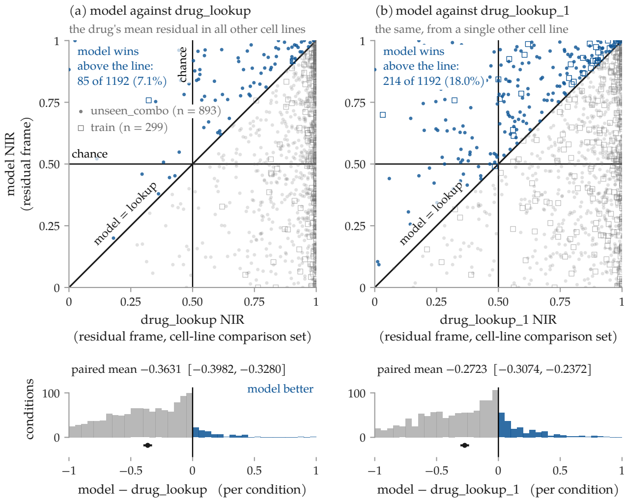
Figure 4.20. The headline gap is a tilt of nearly the whole population and not a mean over a mixed one: the model scores above drug_lookup on 7.1% of conditions, and above the single-cell-line lookup on 18.0%. Every mark is one of the 1,192 conditions of the common support — those on which a training-only lookup exists — and both axes are NIR in the \blacktriangle RESID frame, comparison set other drugs in the same cell line. On this support the model scores 0.549 and the within-well split-half precision reference 0.857; the 1,394-condition figures quoted elsewhere (0.537 and 0.854) are a different population and are not combined with these. (a) Against drug_lookup, the drug's mean residual in all other cell lines, 0.913 pooled: the model is above the identity line on 85 of 1,192 conditions, 7.1%. (b) Against drug_lookup_1, the same quantity from a single other cell line, 0.822 pooled: 214 of 1,192, 18.0%. Marker shape gives the split, 299 train and 893 ? unseen_combo; no unseen_drug condition appears, because no training lookup exists for a drug held out of training, and that regime is therefore not addressed by this figure at all. The lower panels are the per-condition paired difference on a shared count axis, with the paired mean drawn below the counts as a point and bar, the bar a 95% bootstrap interval clustered two-way on cell line and well: -0.3631 [-0.3982, -0.3280] in (a) and -0.2723 [-0.3074, -0.2372] in (b). The win counts are counts over conditions and carry no interval; ties (23 and 28 conditions) count as not a win. The 0.50 rules are chance on both axes, labelled once in (a).
