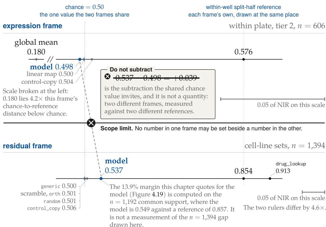
Figure 4.22. The two frames share a chance value and nothing else, and the shared value is exactly what makes the mistake easy. Each scale is stretched so that chance falls at the same place in both and so that each frame's own within-well split-half precision reference falls at the same place as the other's; nothing else is aligned, so the two frames carry different rulers — the same 0.05 of NIR is 4.6\times longer above than below — and that differential stretch is the figure. Upper: the expression frame, within plate, tier 2, n = 606 , where the model scores 0.498 against a reference of 0.576 and is matched by a drug-agnostic linear map (0.500) and a control-copy (0.504); the scale is broken at the left because the global mean, 0.180, lies 4.2\times that frame's chance-to-reference distance below chance. Lower: the residual frame, cell-line sets, n = 1,394 , where the model scores 0.537 against a reference of 0.854, a training-only per-drug lookup reaches 0.913 above that reference, and generic, orth, random and control_copy all fall within 0.006 of chance, one mark at this scale. Both references are within-well split-half precision figures — two disjoint halves of one treated well — and not biological replicates (chapter 3). Chance is 0.50 in both under the exchangeability condition audited in § 4.1, and because it is the one value the two frames share it is exactly what makes the struck-out subtraction in the middle of the figure easy to perform. Every value is a pooled mean drawn as a bare marker; no arm shown here is quoted with an interval at the pooled level, so none is drawn (Table 4.15). The 13.9% margin annotated below is computed on the n = 1,192 common support and is not a measurement of the n = 1,394 gap drawn here.
