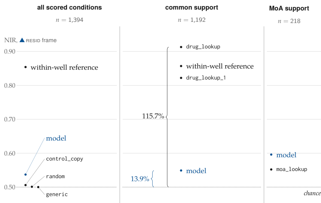
Figure 4.19. A predictor that needs no model, no prompt and no checkpoint scores above the reference the model is measured against, and the three columns may not be read across. Marks are NIR in the ▲ RESID frame, where chance is 0.50. Each column is scored on its own support ( n = 1,394, 1,192 and 218 ), so a mark in one may not be set beside a mark in another; even the reference differs between the first two. On the common support the model covers 13.9% of the distance from chance to the within-well split-half precision reference, and a training-only per-drug lookup covers 115.7% of it, which is a property of the reference and not headroom (Table 4.12). On the MoA support the model scores 0.596 against moa_lookup's 0.552, a +0.0436 the interval does not separate from zero. No interval is drawn: the source gives them on differences between arms, not on the level of one arm, and those are in Table 4.12. Reading the labels: monospace names an arm exactly as Table 4.12 names it, roman names the reference in prose, the accent marks the model, and there is no fourth style. A label a rule would strike or a neighbour would crowd is lifted clear on a hairline; the dot carries the value. Horizontal position inside a column means nothing, and arms whose scores nearly coincide are dodged sideways so each keeps its own dot.
