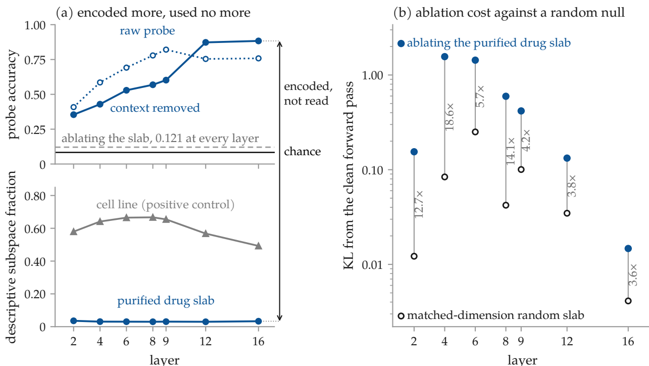
Figure 4.11. Drug-label information becomes more decodable with depth while interventions on the purified slab have limited effect. Layer is a true numeric axis in both panels, so the 9–12–16 spacing is drawn as it is; the two dots at the far left of (b), outside the tick range, are the two direct-label keys and not data. (a) Top : drug-label probe accuracy over twelve drug classes, so chance is 1/12 = 0.083 , on 480 held-out predictions. Two series: the dotted open one is the raw probe, and the solid filled one is the same probe once cell line, plate and dose are projected out. They cross between layers 9 and 12 — removing context lowers decodability at the five shallowest depths and raises it at the two deepest, to 0.873 and 0.883, and this panel is the only place in the document where that is visible. The flat grey line is the same probe after the drug slab is projected out, measured at all seven depths and identical at each. Bottom : the descriptive subspace fraction of the purified drug slab against the cell-line positive control, on its own separate scale — an activation-space summary, not a decomposition of biological drug-response variance. The double-headed arrow at layer 16 joins one point in each half; it marks that the two quantities move apart, and its length measures nothing, the two scales being incommensurable. Encoded, not read names that contrast, but the evidence for not read is panel (b)’s ablation cost and not this panel, which is descriptive throughout. (b) Mean KL from the clean forward pass in nats when the purified drug slab is ablated, against a matched-dimension random slab, n = 60 prompts per entry. Log axis because late-layer divergences are small for everything, and paired dots rather than bars: on a log axis a bar’s length is measured from an arbitrary axis floor, whereas the vertical gap between a pair is their ratio, which is the number annotated beside each pair and the number in Table 4.5. That table’s caveat holds here: the null is matched to the slab’s rank and not to the variance the slab removes — the slab’s subspace fraction runs 4.9 to 7.0 times the null’s, plotted in the lower half of (a) — so the ratio mixes drug content with that difference. The cell-line positive control, against which the ablation cost is 9 to 37% at layers 2 to 9, is not drawn here; Figure 4.10(d) draws it at layer 4 and Table 4.5 carries all seven. No intervals are drawn in either panel, for two different reasons. In (b) the stored dispersions are normal-approximation standard errors over the 60 prompts, not this document’s interval convention (95% bootstrap clustered over cell lines), so as in Table 4.5 this is a sign-and-magnitude reading. In (a) no dispersion was computed at all: the accuracies are stored as bare floats. These accuracies come from a different instrument from the twenty-four-class probe sweep run over the five arms of § 4.5, whose chance is 1/24 on a different label set, and the two must not be read against each other. Whether drug identity is read requires § 4.5.
