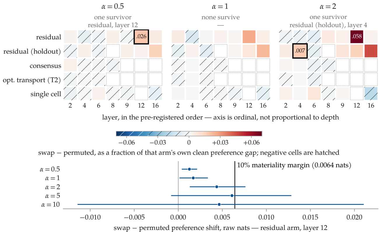
Figure 4.13. The one test that survives multiplicity correction changes arm and depth with the rung of the displacement ladder, and at one rung there is no survivor at all. Each panel is one slice of the ladder: the five training arms of Table A.3 (rows) by the seven probed depths (columns), n = 26 measured tests per slice, on one diverging scale shared across the three panels. Colour is the swap minus permuted effect as a fraction of that arm's own clean preference gap. The layer axis is ordinal, drawn at equal spacing, and is not proportional to depth. Nine of the 35 grid positions were never measured and are drawn as empty dotted outlines, not as zeros. Benjamini–Hochberg is pooled across arms within a slice, as the text applies it and not as the pipeline stores it; q is printed in the three cells that fall below 0.10 and ringed where q < 0.05 . That criterion admits the residual arm at layer 12 at \alpha = 0.5 ( q = 0.026 , on the stored bootstrap draw the text discusses), nothing at \alpha = 1 , and residual_holdout at layer 4 at \alpha = 2 , which demotes layer 12 to q = 0.058 ; it is the only survivor among this chapter's twenty-six headline tests. Beneath, the same residual arm at layer 12 in raw nats across all five rungs, with the 10% pre-registered materiality margin as the vertical rule. Intervals throughout are 95% cluster bootstraps over ordered (A,B) pairs, 4000 resamples, which at this layer is 60 rows in 58 pair clusters over 24 anchor drugs. The three seed replicates are in Table 4.6 and are deliberately not drawn here.
