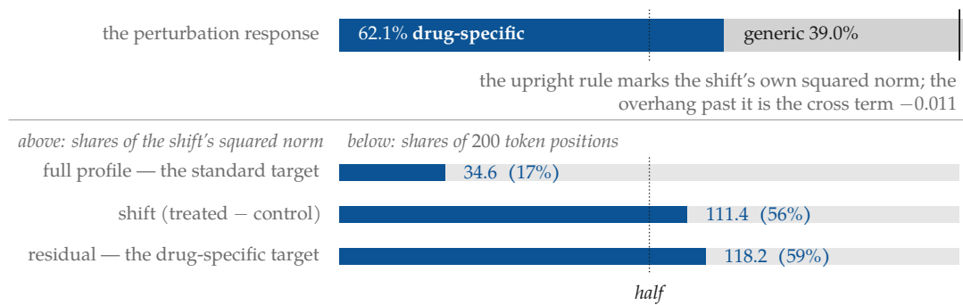
Figure 4.16. The drug is the majority of the perturbation response and almost none of the standard target's tokens. Above the rule: the shift's squared norm decomposes exactly into a drug-specific residual, a generic programme and a cross term, so 62.1% of what a perturbation does to a cell is specific to the drug. Below it: of the 200 positions a cell sentence spends on the standard target, only 34.6 carry a different gene for two drugs in the same context — the other 83% are the same string. Ranking the same measurement by signed residual raises that to 118.2, and at the plate scope this build trains in the residual row reads 120.3 (60%). The two halves of the figure are different quantities, a squared-norm share and a count of token positions; they share the axis and the half-way rule and nothing else, and no difference between them is a number. What the picture states is an ordering: the signal is a majority of the response, the standard encoding exposes a small minority of it to the loss, and the residual encoding puts the exposed fraction back on the majority side (Table 4.8).
