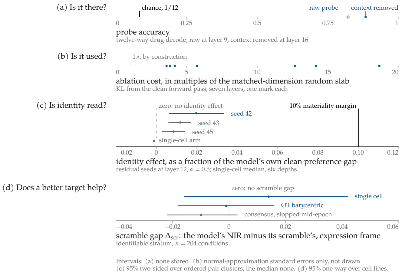
Figure 4.7. Each instrument answers a different question against a different comparator, and the four rules may not be read across. The four rules share a length and both endpoints and nothing else: each carries its own quantity, named beneath it, and its own comparator. The zeros of (c) and (d) are deliberately not vertically aligned, since aligning them would assert the commensurability this figure exists to deny. Converting one rule into another is the inference this part exists to block. Where an instrument returns a clustered bootstrap its mark carries a bar; where it does not, the mark sits bare on the rule, and the foot line names the construction row by row. (a) The two accuracies are at different depths and are not a before-and-after pair: the open mark is the raw probe at layer 9, the filled one the same probe at layer 16 once cell line, plate and dose are projected out. The two series cross between layers 9 and 12 — removing context raises accuracy at the two deepest probes — and only Figure 4.11(a), which has a layer axis, can show it. The floor is analytic, not empirical: workspace_probe.json stores chance as exactly 1/12 and holds no permutation null. What projecting the drug slab out costs this probe belongs to Figure 4.9 and Figure 4.11(a) and is not drawn here. (b) The seven marks are the seven probed depths in value order and are not identified; which mark is which layer is Figure 4.11(b), which plots both divergences against a numeric layer axis, and the Ratio column of Table 4.5. That table's caveat holds here too: the null is matched to the slab's rank and not to the variance the slab removes, the slab's subspace fraction running 4.9 to 7.0 times the null's, so the ratio mixes drug content with that difference. (c) The three seeds are the first three rows of Table 4.6, and the black rule is the 10% materiality margin pre-registered for calling an effect material, drawn in the same weight and colour as in Figure 4.13 and Figure 4.12. Layer 12 is the anchor seed's maximum over its seven depths and the only one whose interval excludes zero; a fourth replicate, seed 44, stores swap_skipped at layer 12 and is not drawn. The single-cell mark is a median over that arm's six measured depths — layer 12 is skipped there, its cell-line headroom of 3.88 falling below the 5\times gate — and no interval is stored for a median, which is why it carries none. (d) The comparator is zero and not chance, the quantity being a difference against the model's own scrambled partner on the identifiable stratum in the expression frame (Table 4.7); the consensus arm is greyed because its run was stopped mid-epoch.
