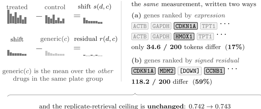
Figure 7: The information was always present; the tokenisation discarded it. Left: the drug-specific residual is built by two subtractions. The control removes the cell’s own state, leaving the shift ; the mean over the other drugs in the same plate group removes the generic programme that every compound triggers, leaving what makes this drug different. Right: that same measurement, written two ways. Ranking genes by expression (a) puts housekeeping genes first, so only 34.6 of the top 200 tokens differ between two drugs in the same context; ranking by signed residual (b) raises that to 118.2. (Divergence counts quoted at cell-line scope, as in Table 9; plate scope is similar.) The bracket is the point of the figure — the replicate-retrieval ceiling is essentially identical under both encodings, so no information has been added. What changed is how much of it the token sequence exposes to the loss.
