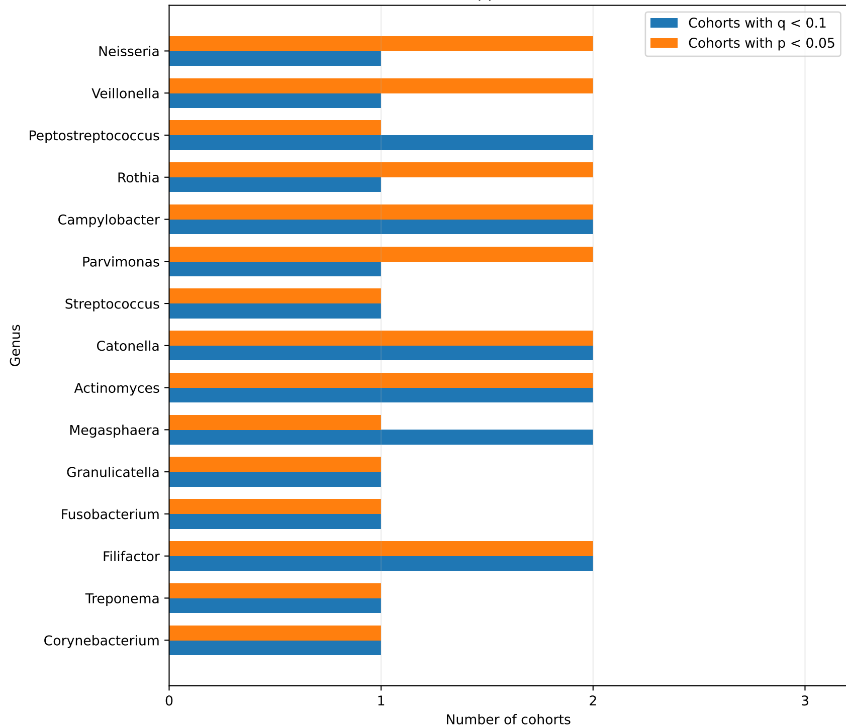
Statistical support across cohorts
