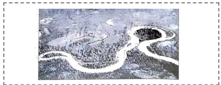
Erosional work of river
