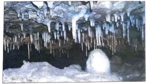
Depositional work of groundwater
