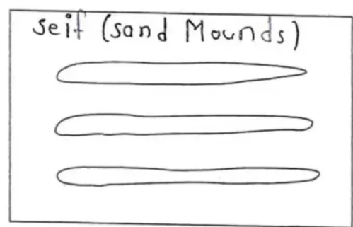
Seif (sand mounds)
