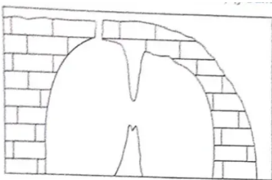
Stalactite and stalagmite cave
