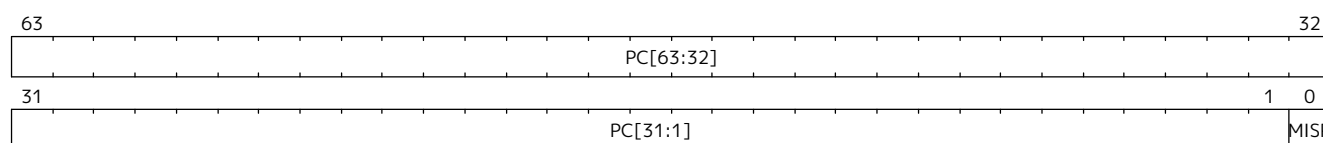
Figure 130. Control Transfer Record Target Register Format for MXLEN=64
