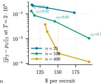
(c) margin threshold c_0
