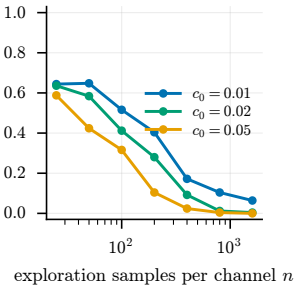
(a) P(p_G \notin \text{true hull of } \hat{I})
