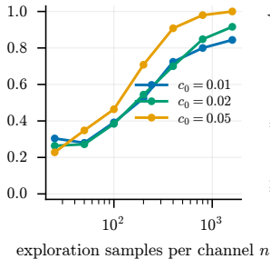
(b) P(c(\hat{I}) \geq c_0/2)
