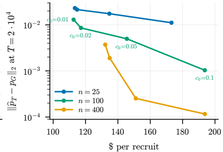
(c) margin threshold c_0
