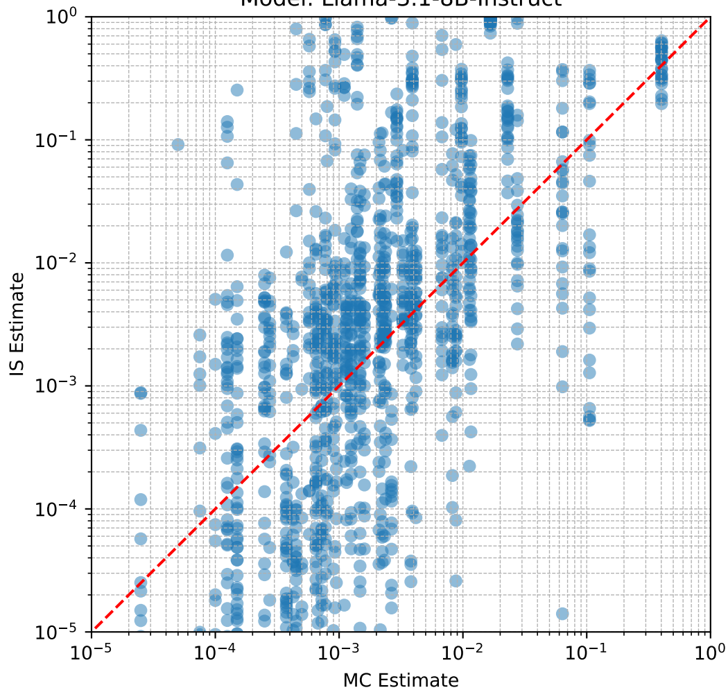
Model: Llama-3.1-8B-Instruct
