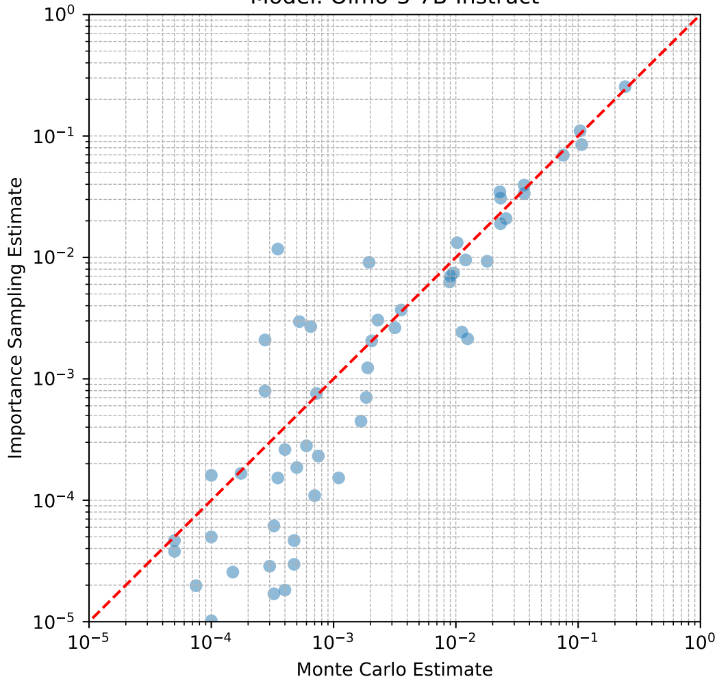
Model: Olmo-3-7B-Instruct
