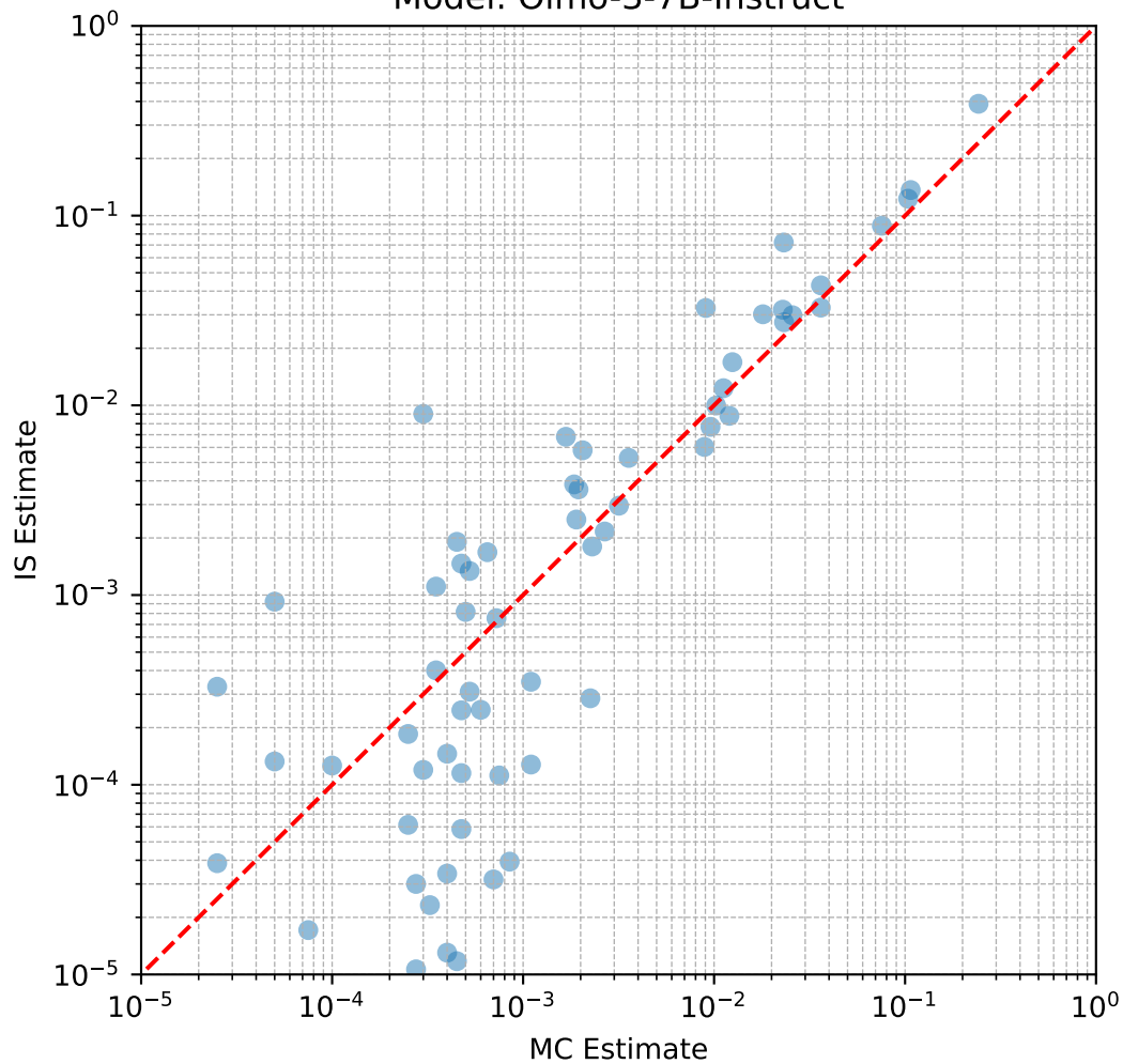
Model: Olmo-3-7B-Instruct
