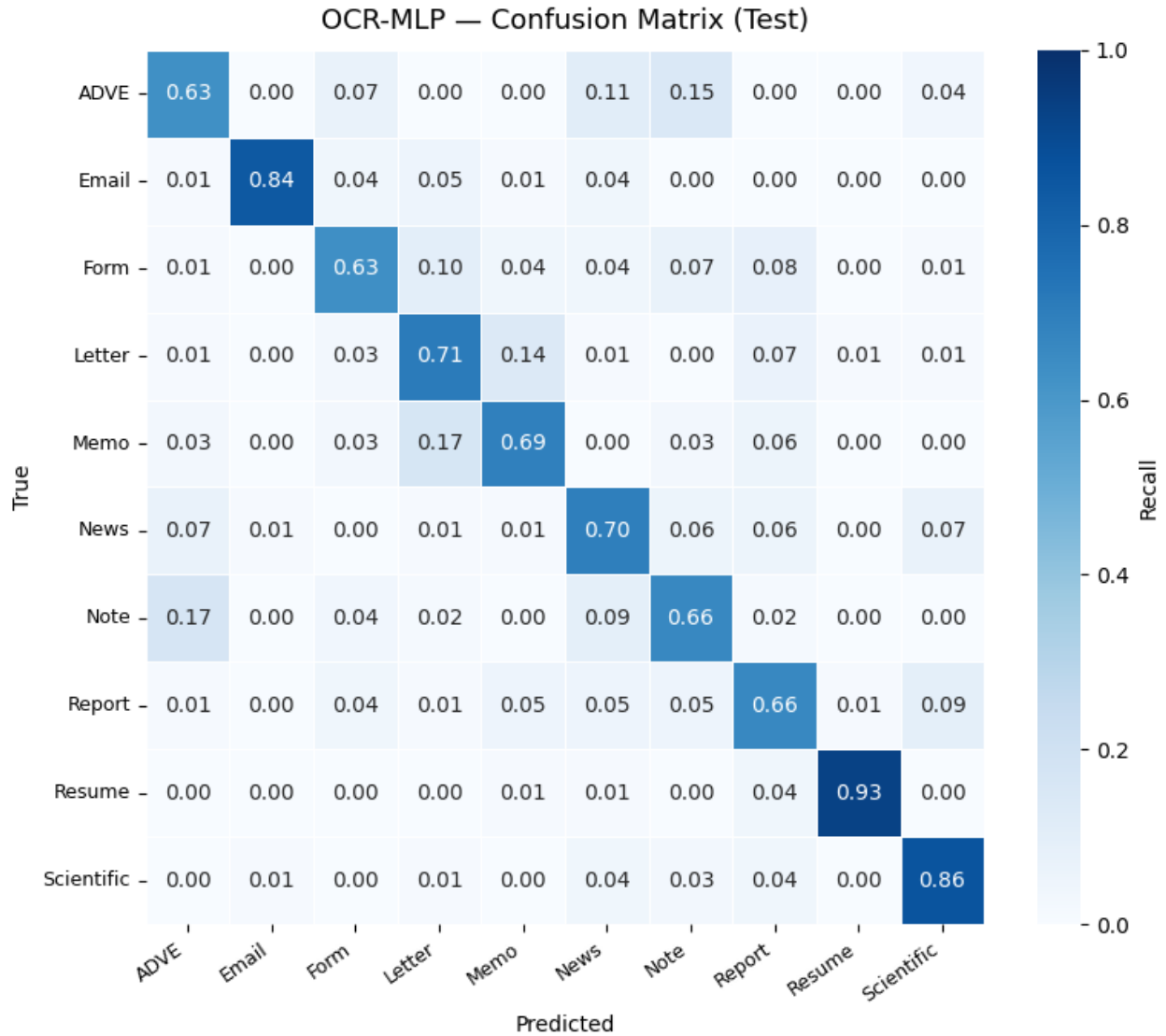
Figure 8: OCR-MLP Confusion Matrix on Test Set (10 Document Classes)
