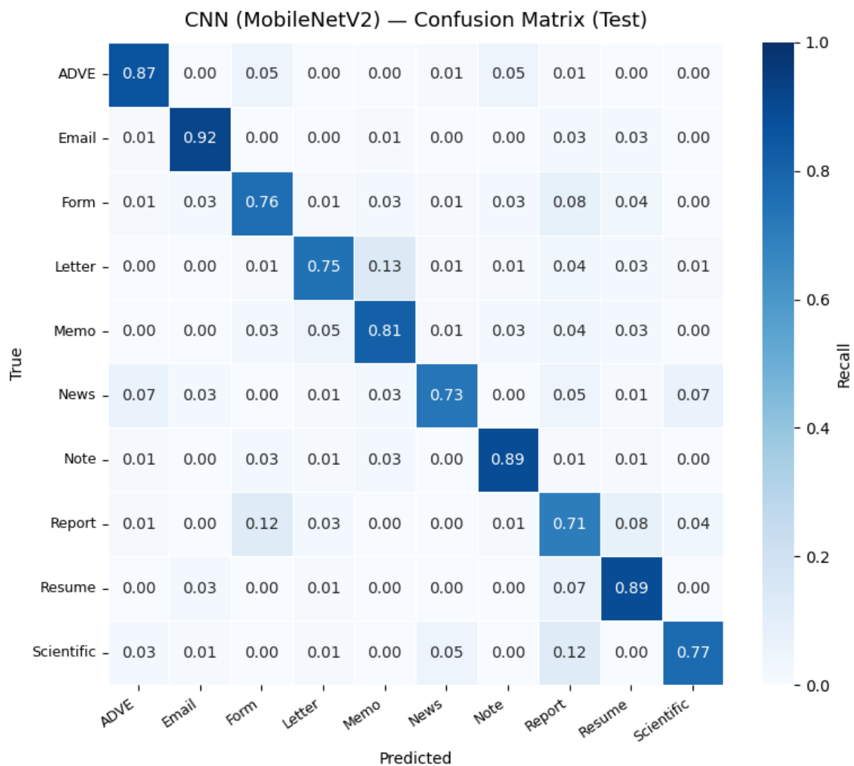
Figure 7: CNN (MobileNetV2) Confusion Matrix on Test Set (10 Document Classes)
