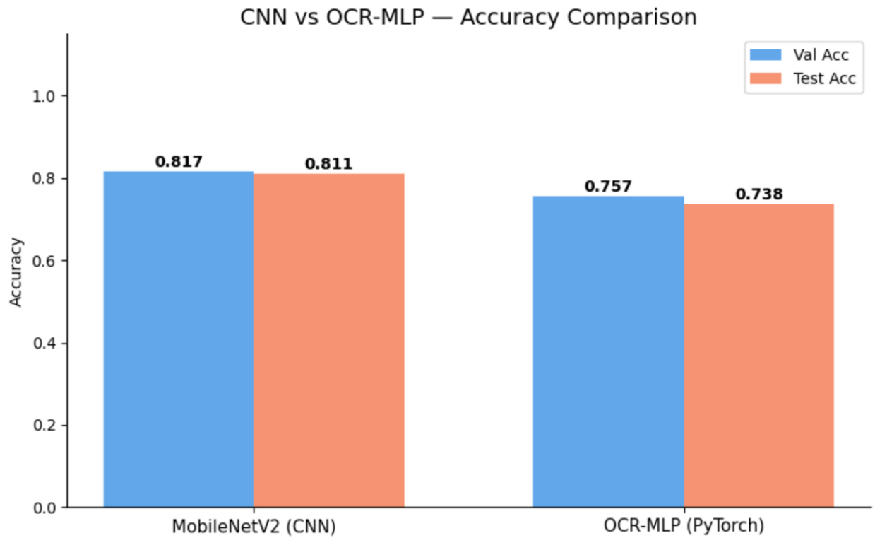
Figure 9: CNN (MobileNetV2) vs OCR-MLP Accuracy Comparison on Validation and Test Sets
