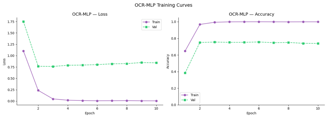
Figure 5: OCR-MLP Training Curves: Loss and Accuracy over 10 Epochs (Train vs Val) — showing Overfitting
