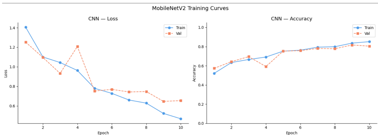
Figure 2: CNN Training Log: Epoch-by-Epoch Train and Validation Loss/Accuracy — Best Val Accuracy: 0.8168
