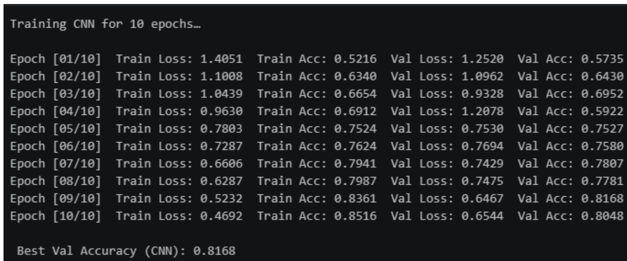
Figure 2: CNN Training Log: Epoch-by-Epoch Train and Validation Loss/Accuracy — Best Val Accuracy: 0.8168
