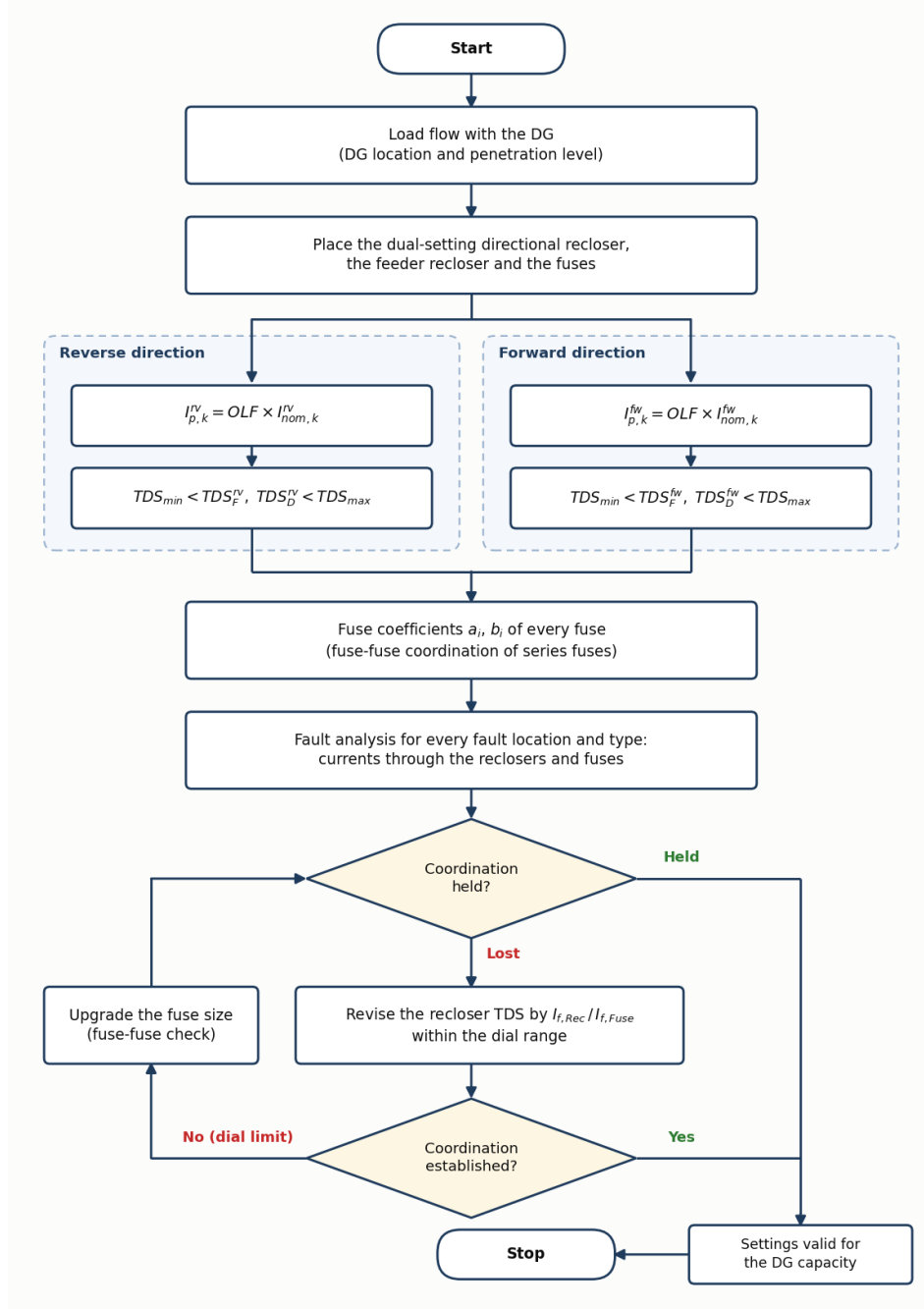
Figure 2: Flowchart of the recloser–fuse coordination method with the DSDR.
