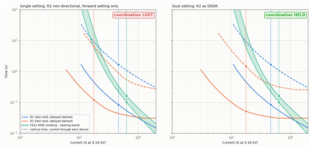
Figure 14: Three-phase fault at 10 % of line 632–633: single setting (left) and dual setting (right).
