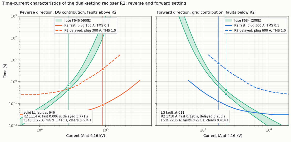
Figure 10: The two setting groups of R2: reverse (DG contribution, faults towards 632) and forward (grid contribution, faults beyond 671), each with one fault of the model.
