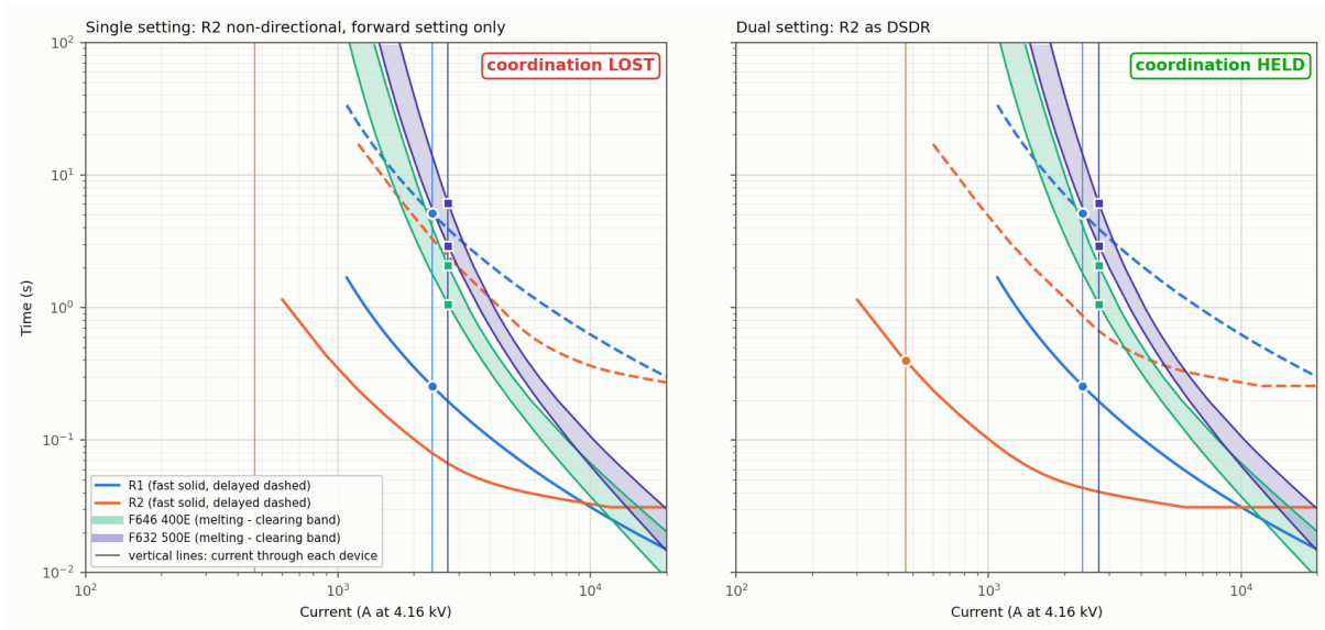
Figure 15: LG fault at 646: the single-setting R2 does not pick up the reverse current; the reverse group does.
