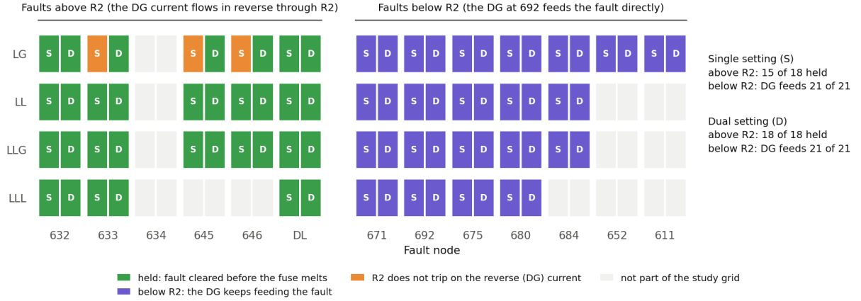
Figure 16: Time-sequence check of all 39 cells: in each cell S is the single setting and D the dual setting on R2.
