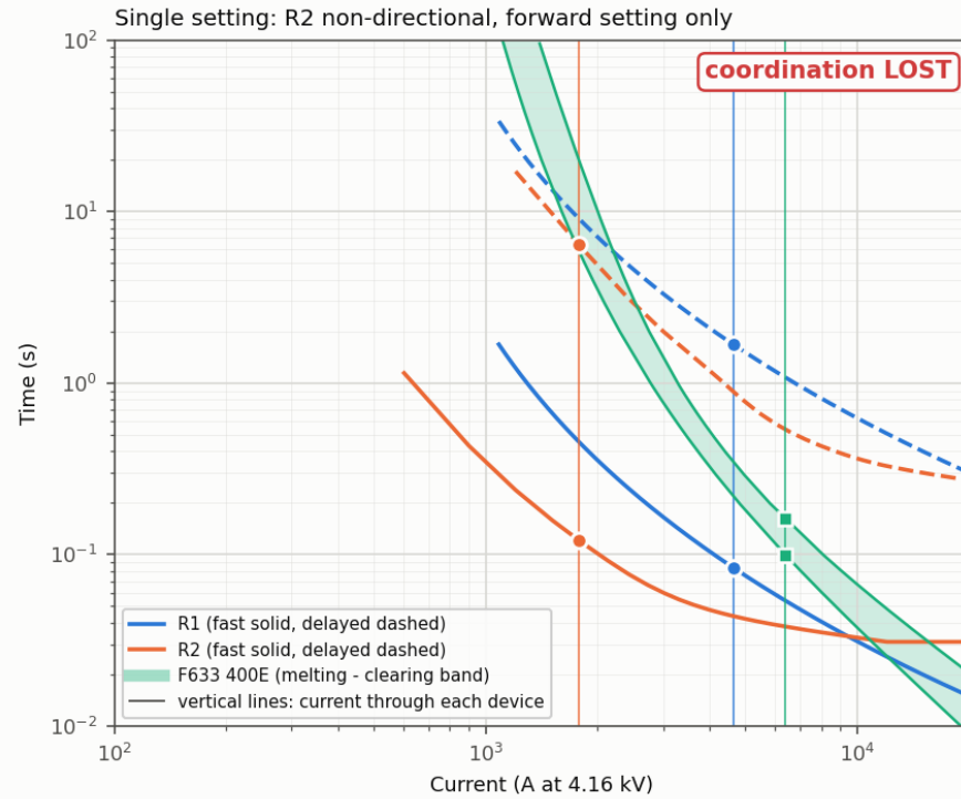
Case 05 - 3-phase fault at 10 % of 632-633, Z_f = 0 ohm (bolted), DG 4.05 MVA connected at 692 (Fig. 13)
