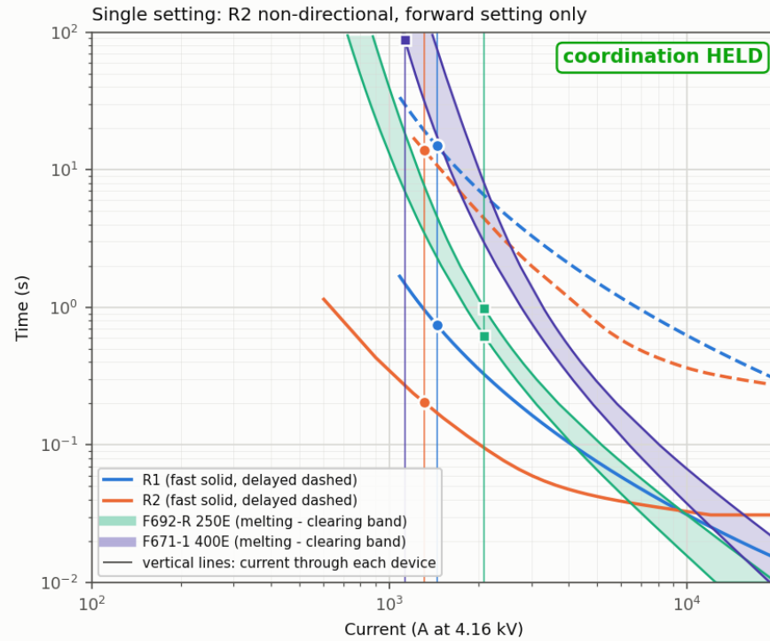
Case 02 - LLG fault at the middle of 692-675, Z_f = 1.0 ohm, DG 4.05 MVA connected at 692 (Fig. 9)
