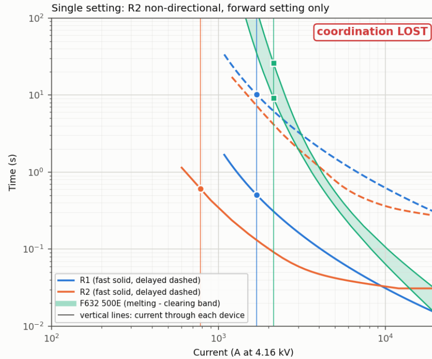
Case 04 - LL fault at 645, Z_f = 1.5 \text{ ohm} , DG 4.05 MVA connected at 692 (Fig. 12)
