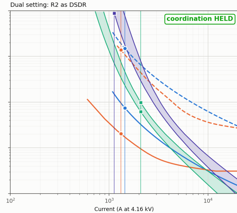
Case 02 - LLG fault at the middle of 692-675, Z_f = 1.0 ohm, DG 4.05 MVA connected at 692 (Fig. 9)
