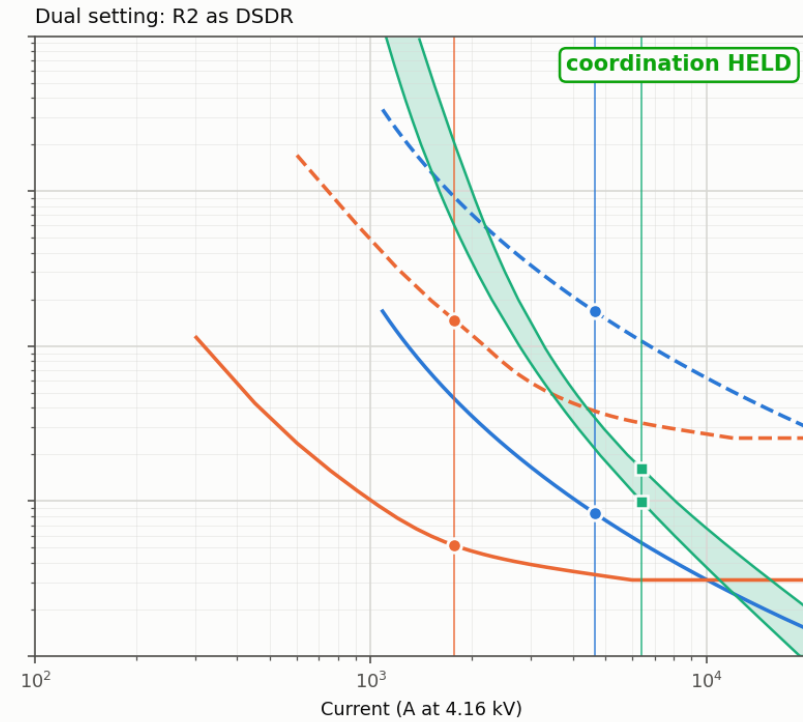
Case 05 - 3-phase fault at 10 % of 632-633, Z_f = 0 ohm (bolted), DG 4.05 MVA connected at 692 (Fig. 13)
