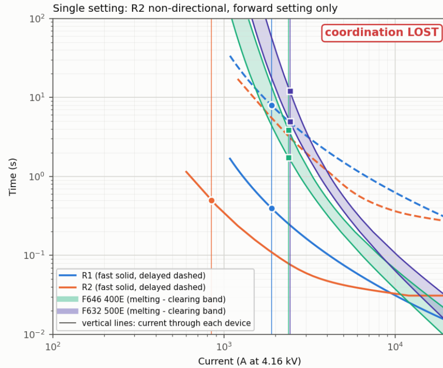
Case 03 - LL fault at 646, Z_f = 1.0 ohm, DG 4.05 MVA connected at 692 (Fig. 11)
