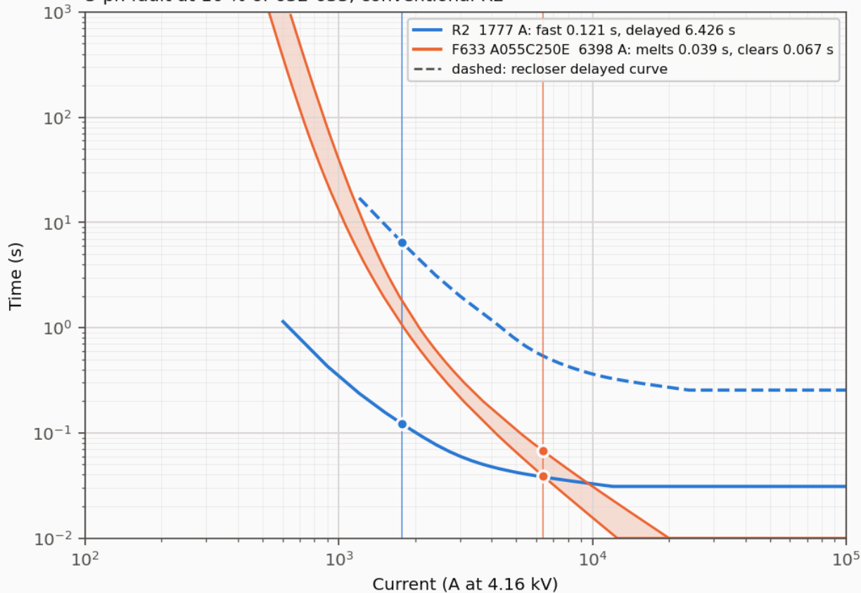
3-ph fault at 10 % of 632-633, conventional R2
