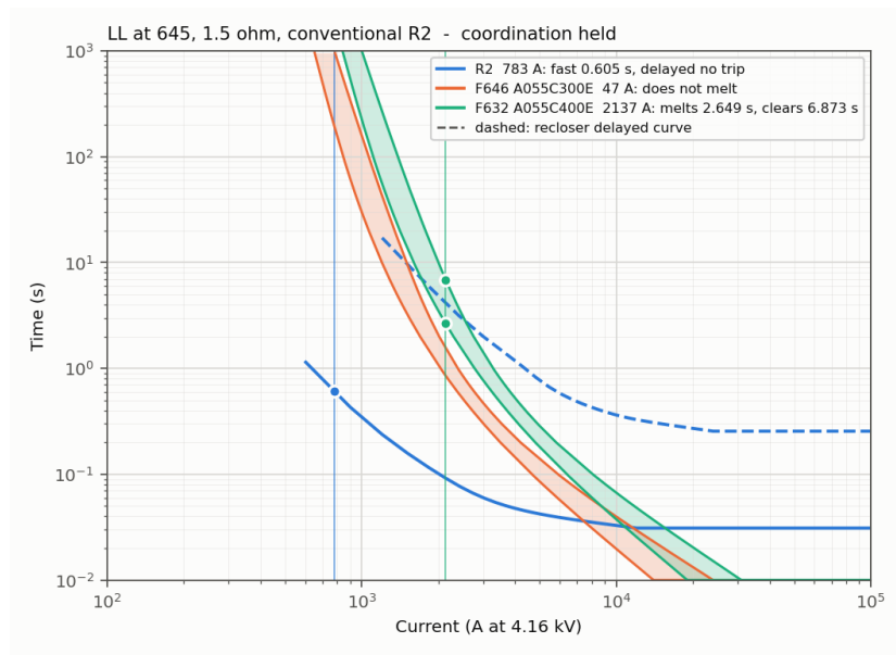
Figure 7: LL fault at 645 through 1.5 \Omega , conventional R2.
