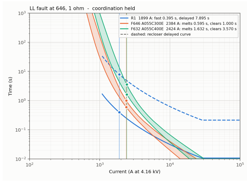
Figure 6: LL fault at 646 through 1 \Omega : R1 with F646 and F632.
