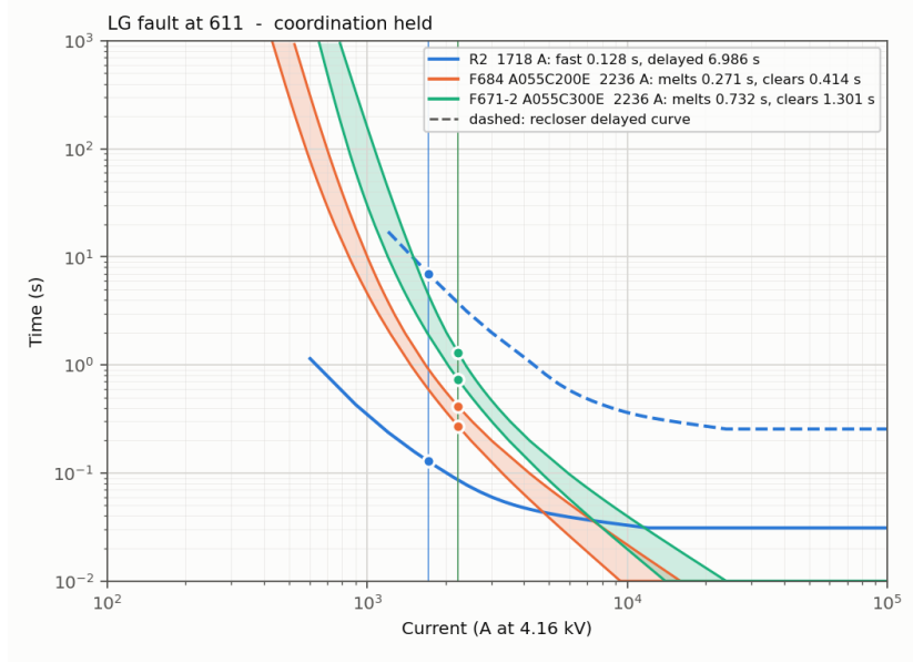
Figure 3: LG fault at 611: R2 forward, fuses F684 and F671-2.
