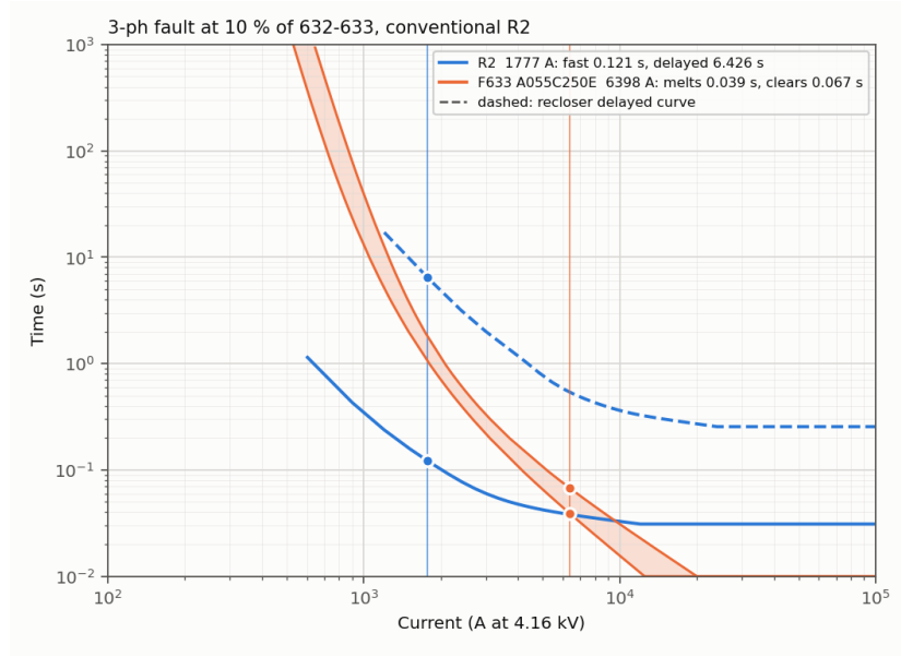
Figure 8: Three-phase fault at 10 % of line 632–633, conventional R2.
