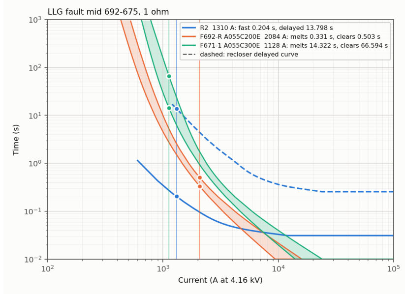
Figure 4: LLG fault at the middle of 692–675 through 1 \Omega .
