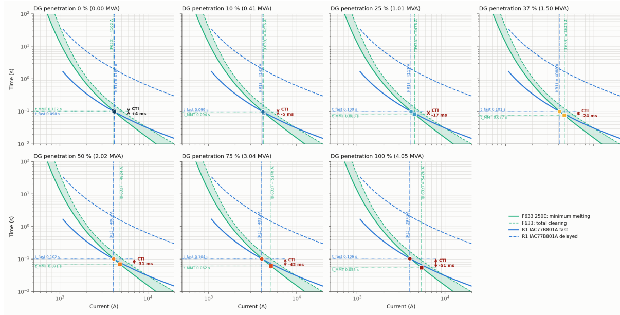
Figure 20: Node 633, fuse F633 and R1, at each penetration level, with the short-circuit currents, operating times and CTI.
