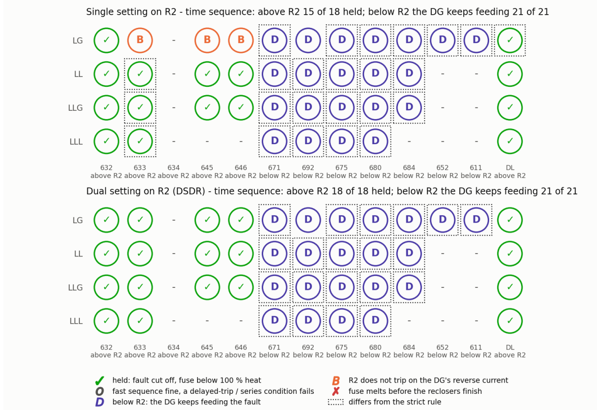
Figure 15: Time-sequence check of all 39 cells, single against dual setting.
