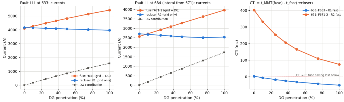
Figure 18: Currents through the fuse (grid and DG share), the recloser (grid share) and from the DG, and the resulting CTI, against DG penetration.
