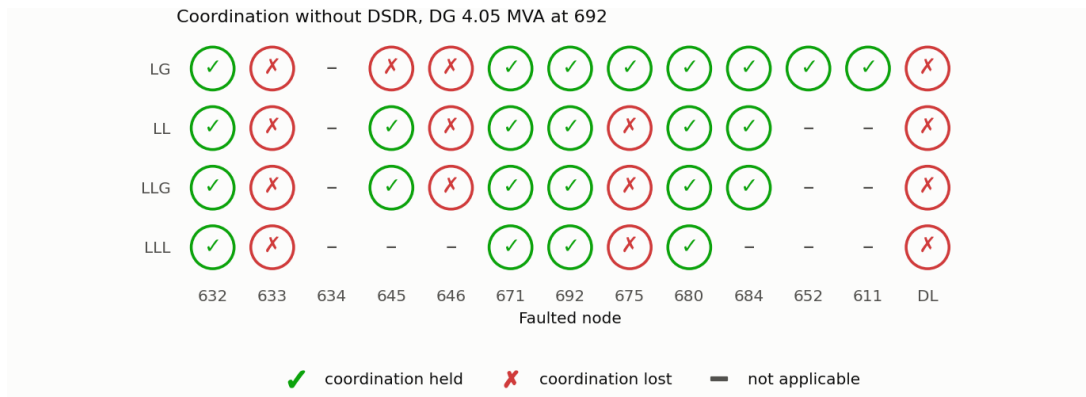
Figure 5: Coordination status with DG, without the DSDR.
