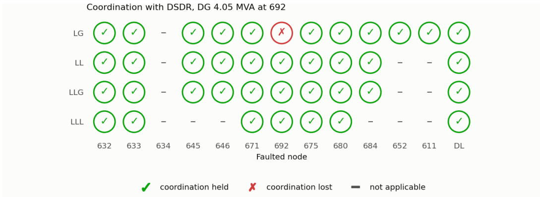
Figure 10: Coordination status with DG and the DSDR.
