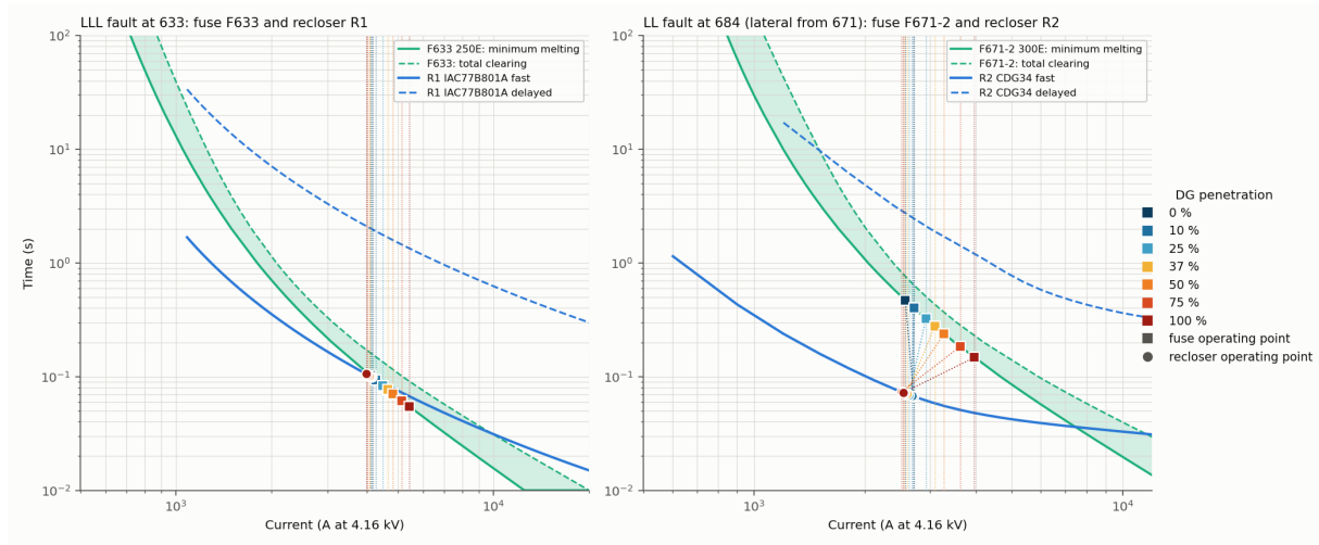
Figure 19: Time–current characteristics at all penetration levels: fuse operating points (squares) and recloser operating points (circles).
