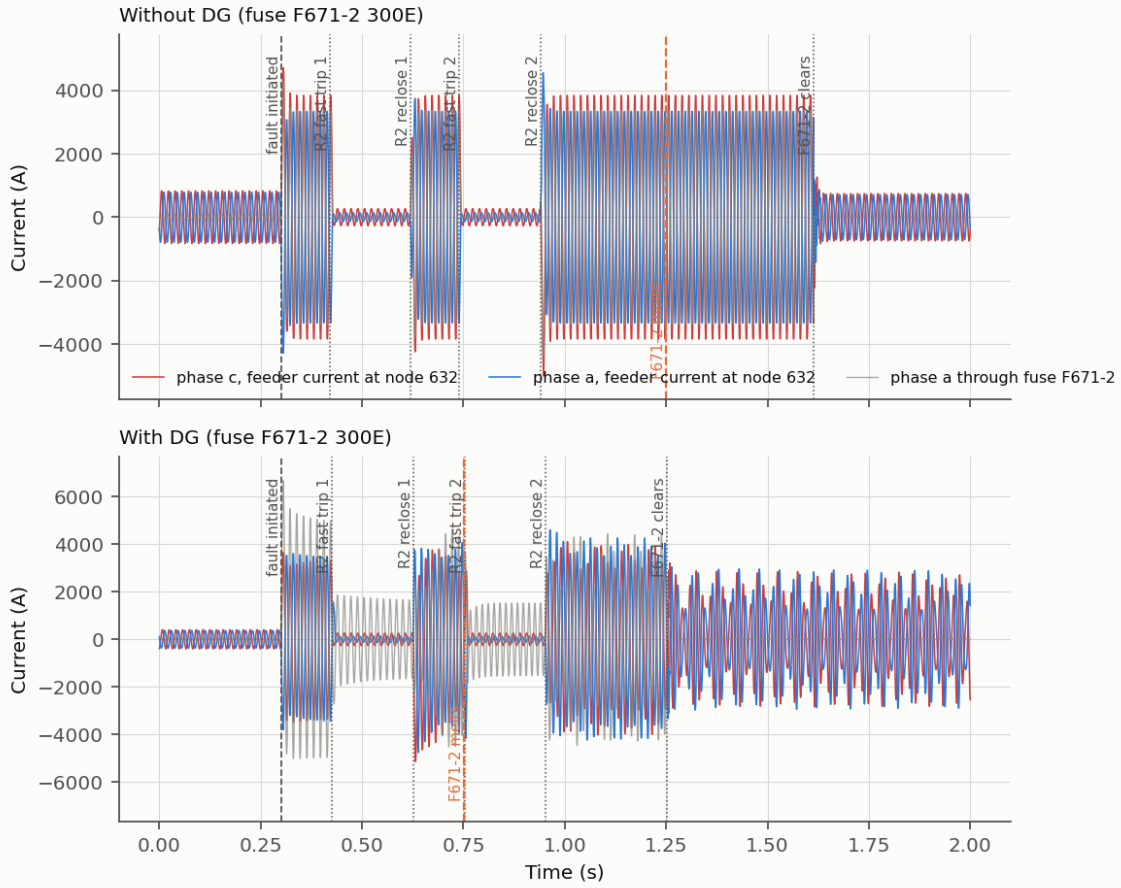
Figure 16: Time-domain current at node 632 for an LL (a-c) fault at 684 through 0.2 \Omega : without DG (top) and with DG (bottom).
