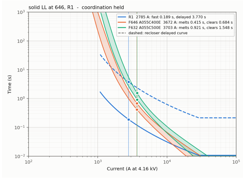
Figure 12: Bolted LL fault at 646: R1 with F646 and F632.
