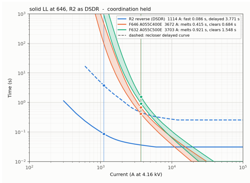
Figure 11: Bolted LL fault at 646: R2 reverse setting with F646 and F632.
