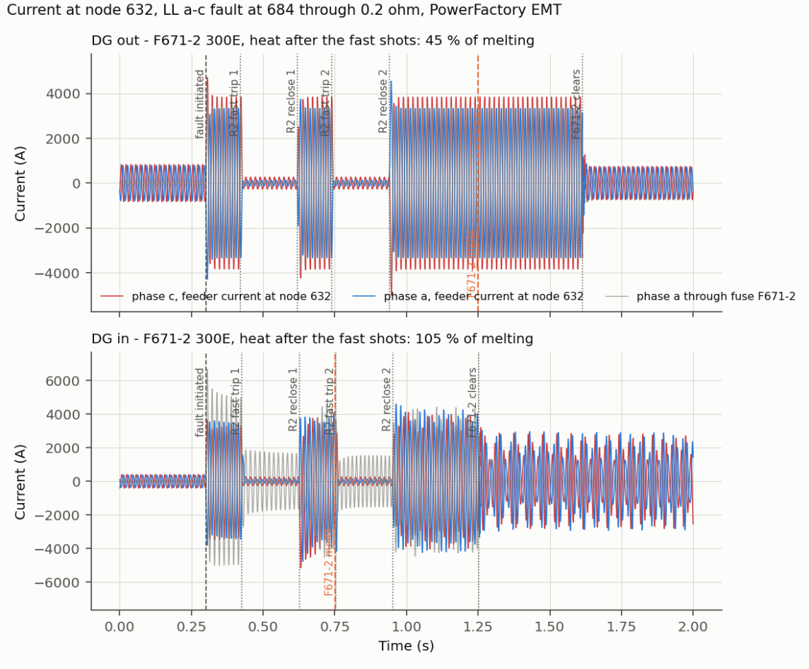
Figure 17: Time-domain current at node 632 for an LL (a-c) fault at 684 through 0.2\ \Omega : without DG (top) and with DG (bottom).
