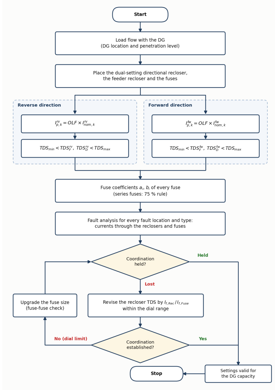
Figure 2: Flowchart of the recloser–fuse coordination method with the DSDR (adapted from [1]).
