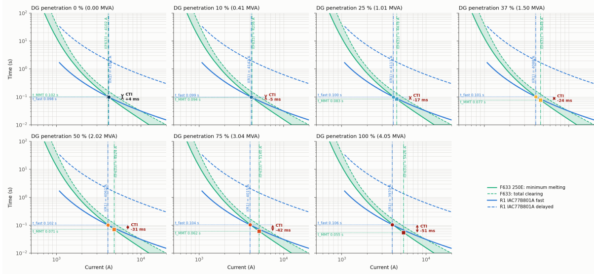
Figure 21: Node 633, fuse F633 and R1, at each penetration level, with the short-circuit currents, operating times and CTI.
