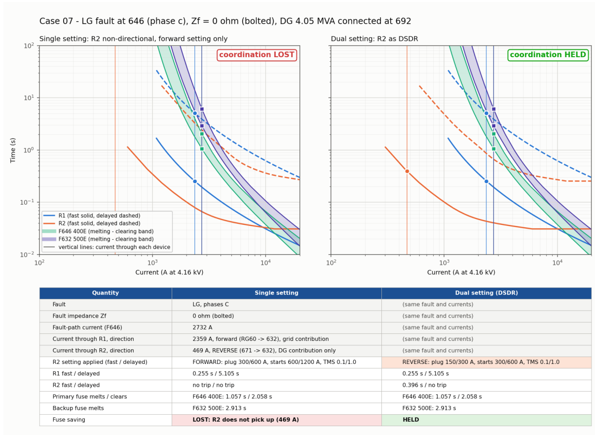
Figure 15: LG fault at 646: the single-setting R2 does not pick up the reverse current; the reverse group does.
