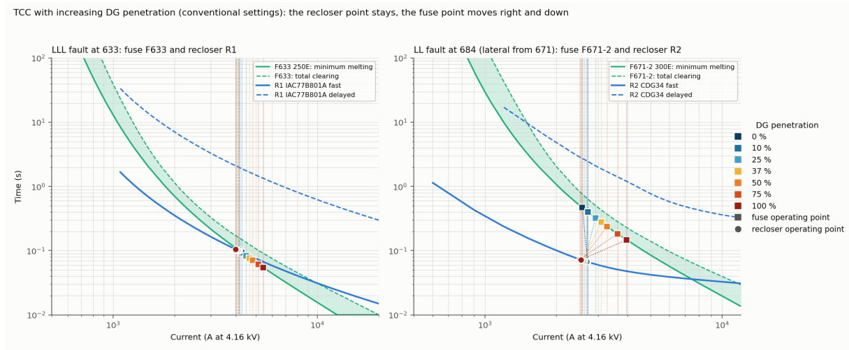
Figure 20: Time–current characteristics at all penetration levels: fuse operating points (squares) and recloser operating points (circles).
