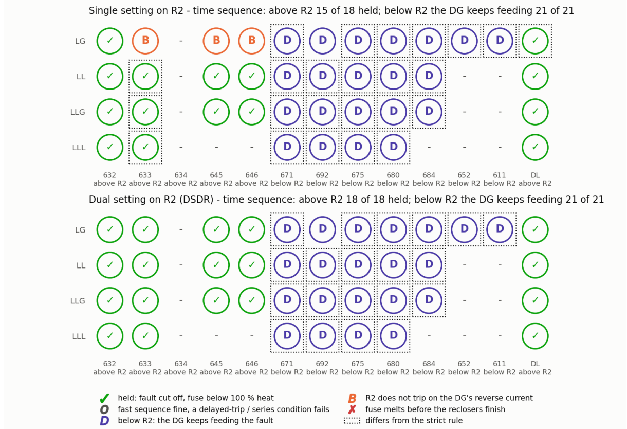
Figure 16: Time-sequence check of all 39 cells, single against dual setting.
