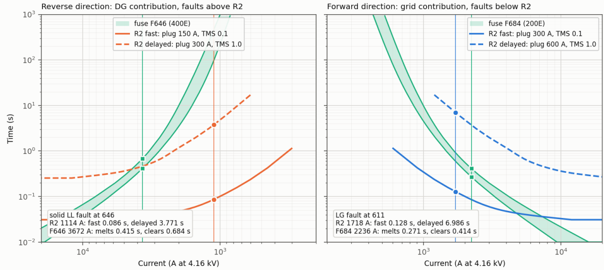
Time-current characteristics of the dual-setting recloser R2: reverse and forward setting
