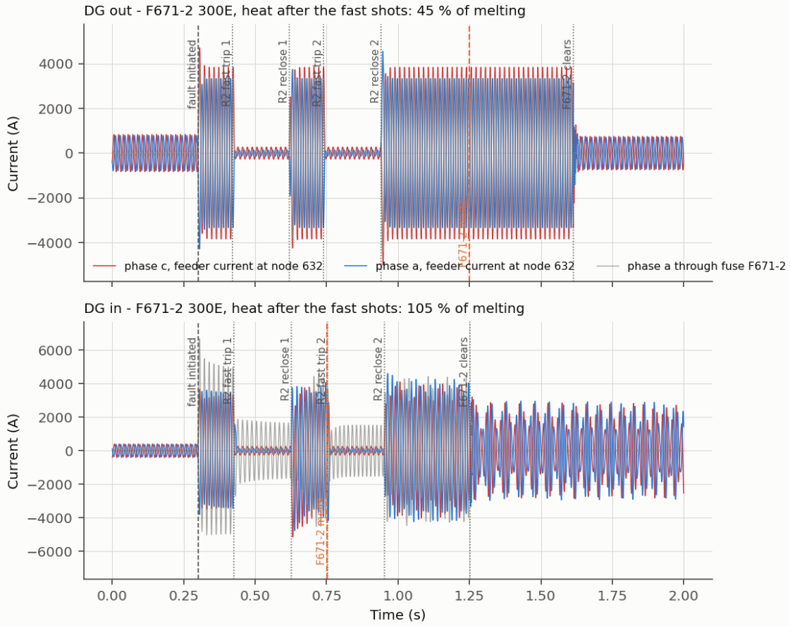
Figure 17: Time-domain current at node 632 for an LL (a-c) fault at 684 through 0.2 \Omega : without DG (top) and with DG (bottom).
