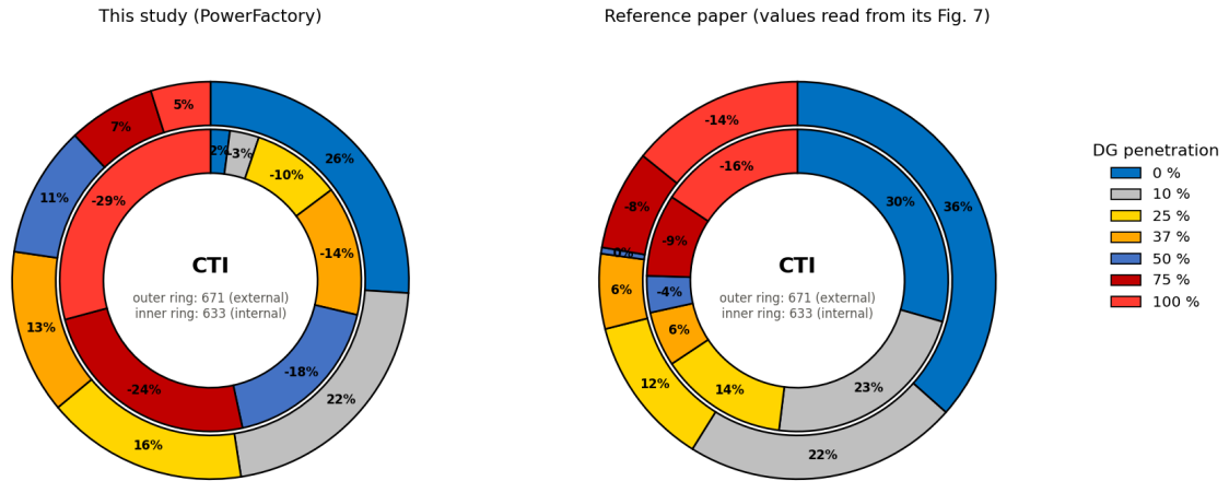
Figure 22: CTI against DG penetration: this study (left) and the values read from the paper's Fig. 7 (right).
