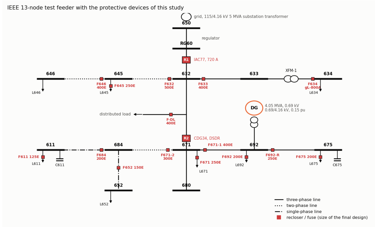
Figure 3: IEEE 13-node feeder with the reclosers R1 and R2, the fuses and the DG at node 692.
