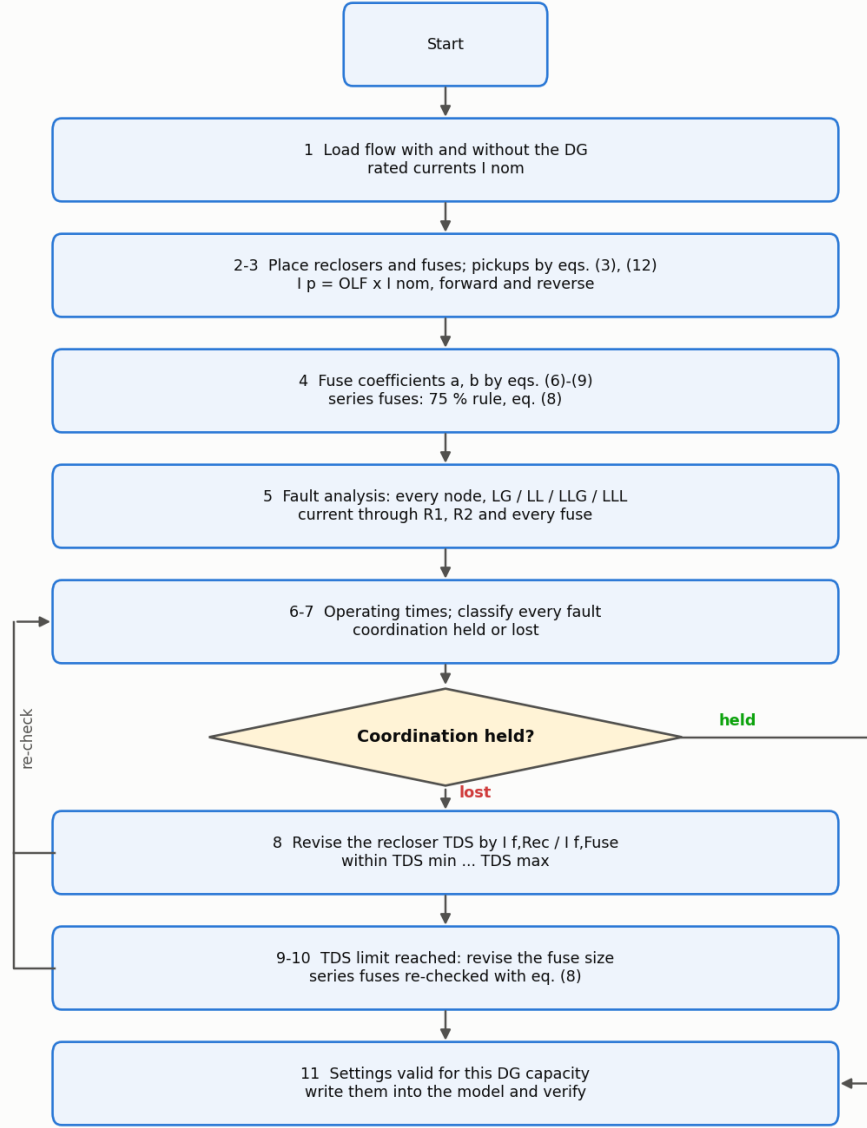
Recloser-fuse coordination method with the DSDR
