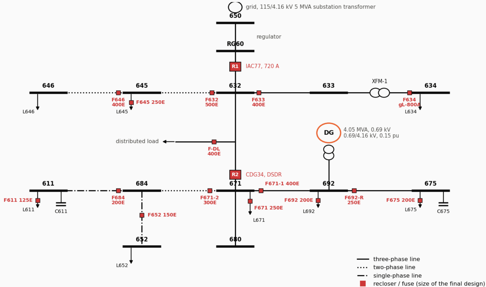
Fig. 6 - IEEE 13-node test feeder with the protective devices of this study
