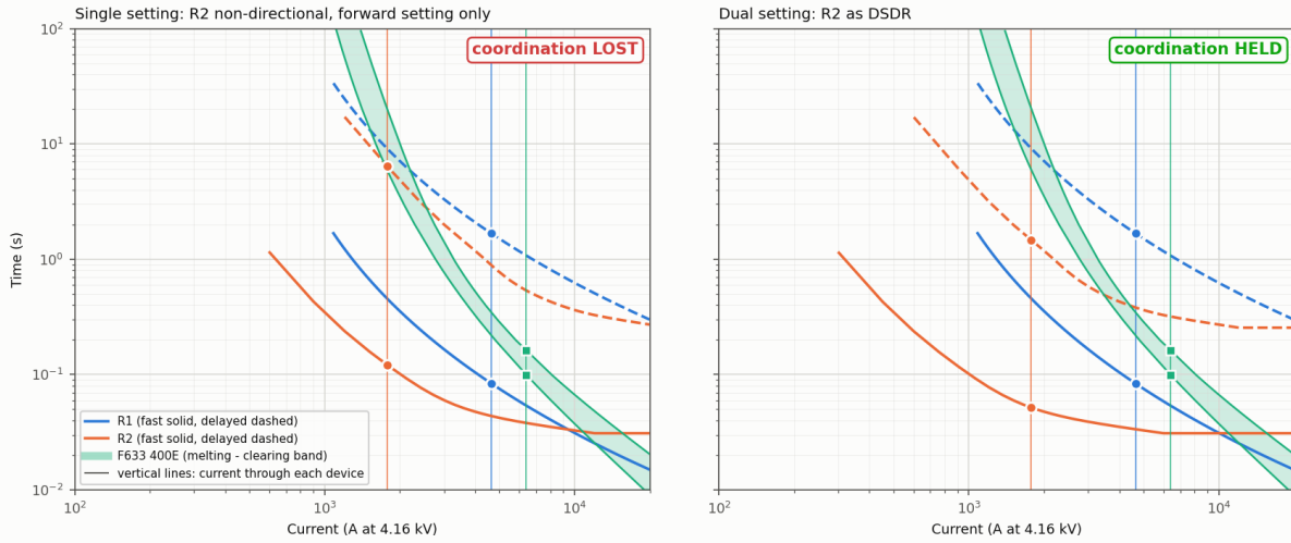
Case 05 - 3-phase fault at 10 % of 632-633, Z_f = 0 ohm (bolted), DG 4.05 MVA connected at 692 (Fig. 13)
