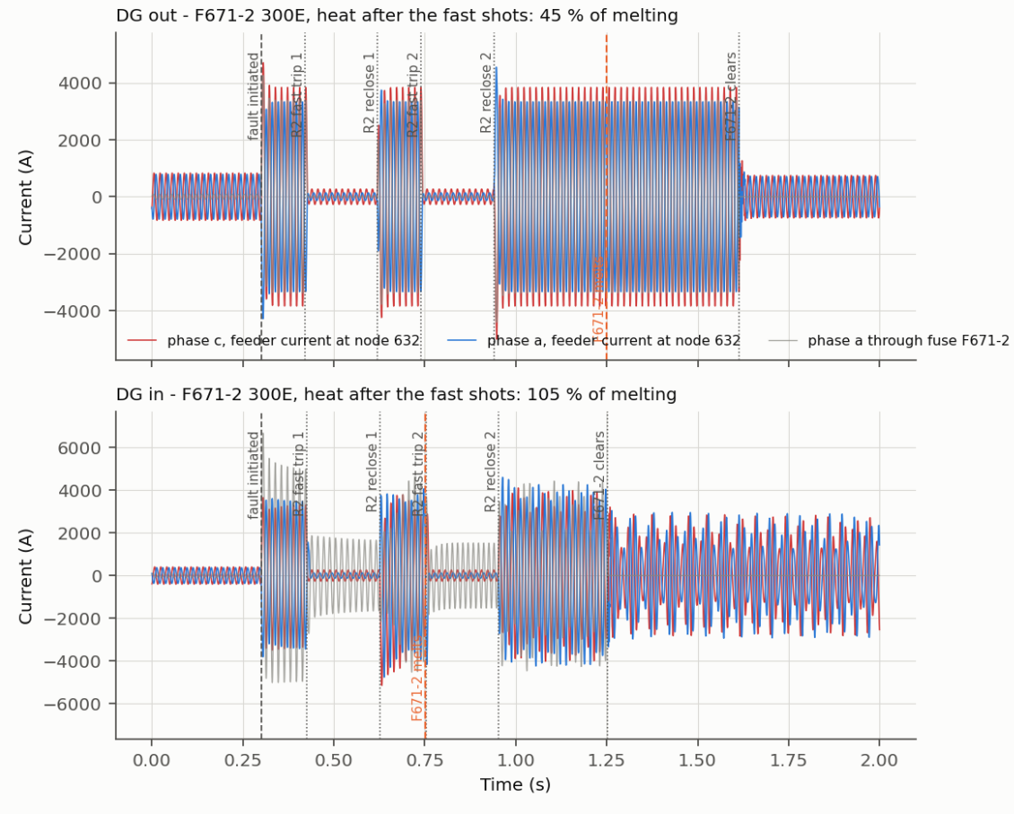
Figure 18: Time-domain current at node 632 for an LL (a-c) fault at 684 through 0.2\ \Omega : without DG (top) and with DG (bottom).
