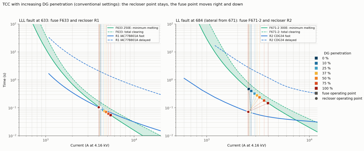
Figure 21: Time–current characteristics at all penetration levels: fuse operating points (squares) and recloser operating points (circles).
