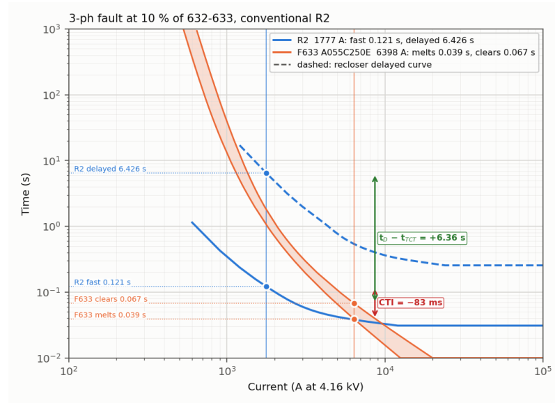
Figure 5.6 Three-phase fault at 10 per cent of line 632–633, conventional R2; CTI = -83 \text{ ms} , the fuse melts first.
