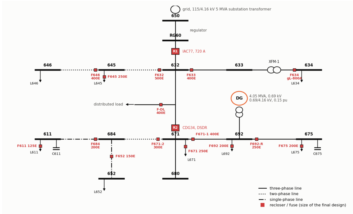
Figure 2: IEEE 13-node feeder with the reclosers R1 and R2, the fuses and the DG at node 692.
