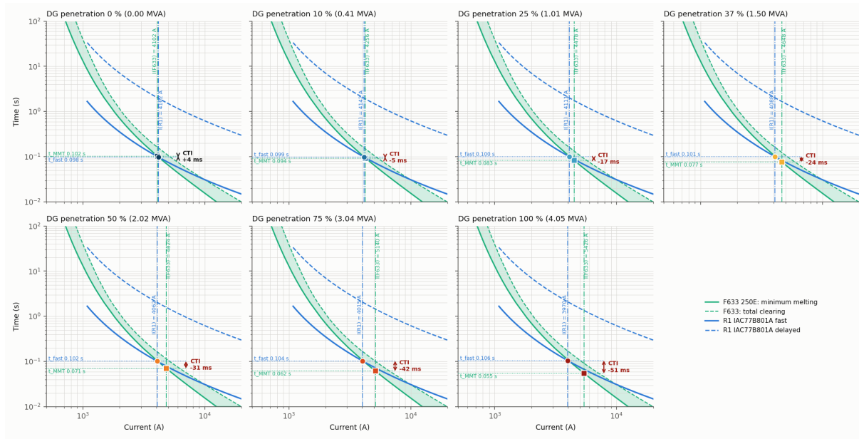
Figure 20: Node 633, fuse F633 and R1, at each penetration level, with the short-circuit currents, operating times and CTI.
