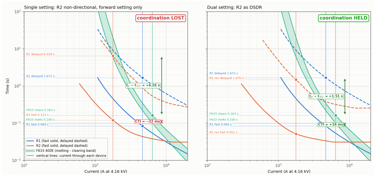
Figure 13: Three-phase fault at 10 % of line 632–633: single setting (left, CTI = –22 ms) and dual setting (right, CTI = +16 ms).
