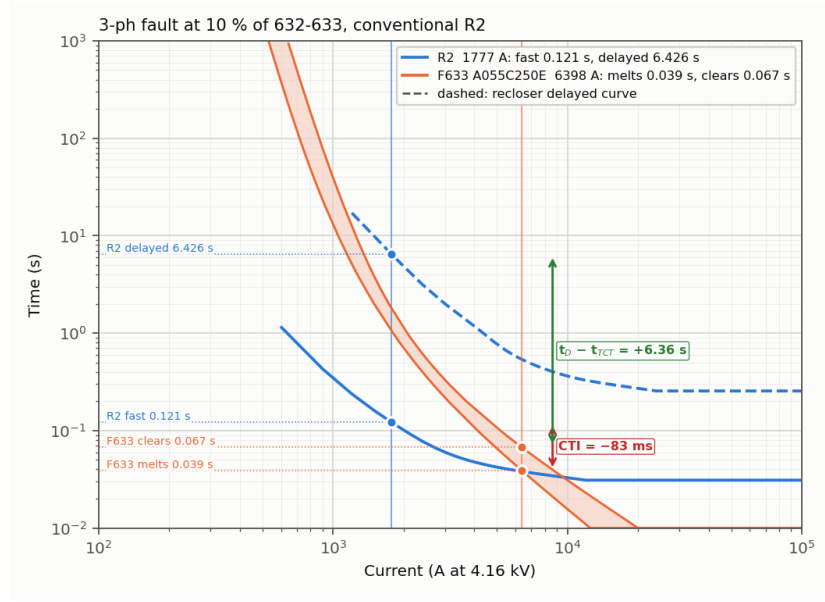
Figure 8: Three-phase fault at 10 % of line 632–633, conventional R2; CTI = –83 ms, the fuse melts first.
