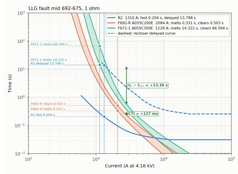
Figure 4: LLG fault at the middle of 692–675 through 1 \Omega ; CTI = +127 ms.
