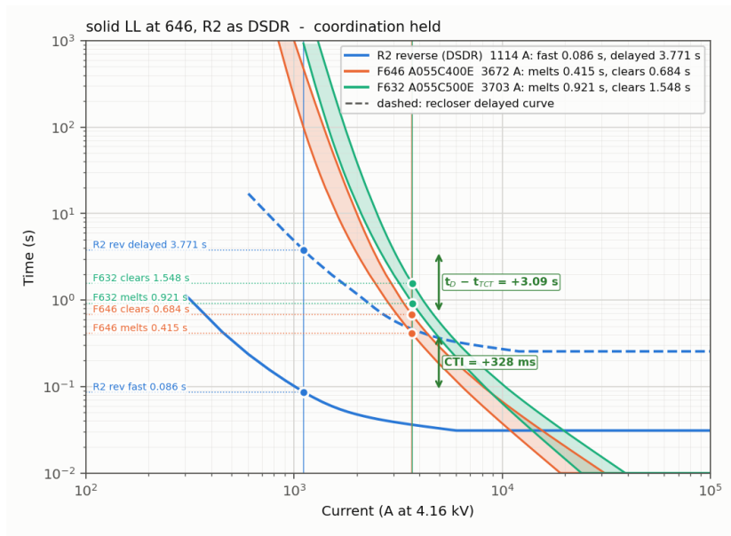
Figure 11: Bolted LL fault at 646: R2 reverse setting with F646 and F632; CTI = +328 ms.
