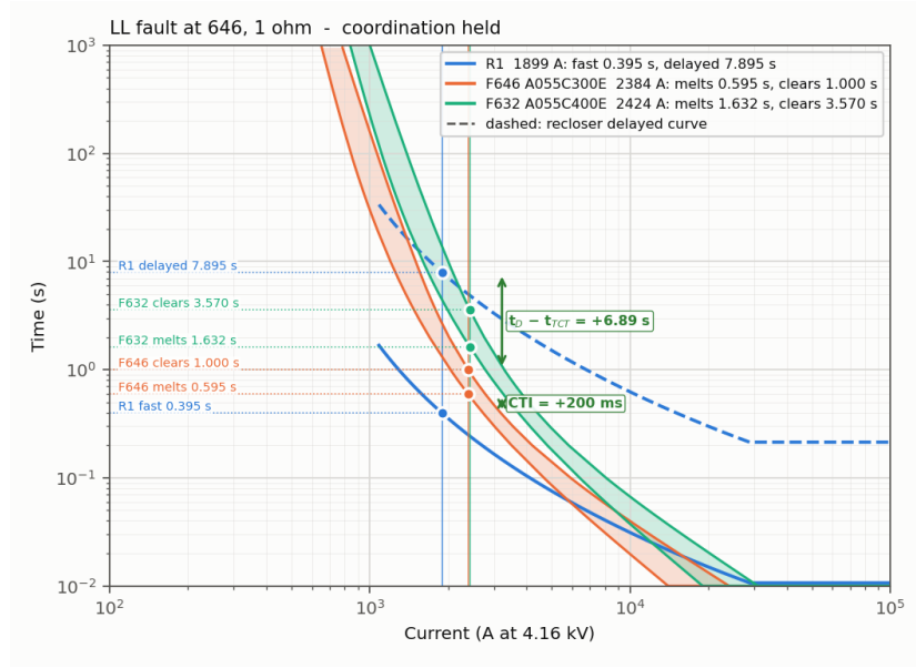
Figure 6: LL fault at 646 through 1 \Omega : R1 with F646 and F632; CTI = +200 ms.
