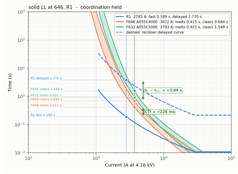
Figure 12: Bolted LL fault at 646: R1 with F646 and F632; CTI = +226 ms.
