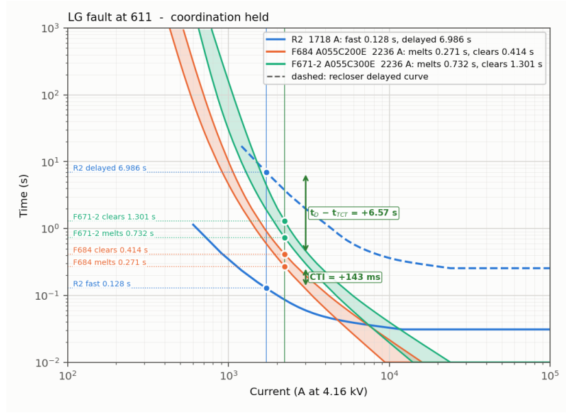
Figure 3: LG fault at 611: R2 forward, fuses F684 and F671-2; CTI = +143 ms.
