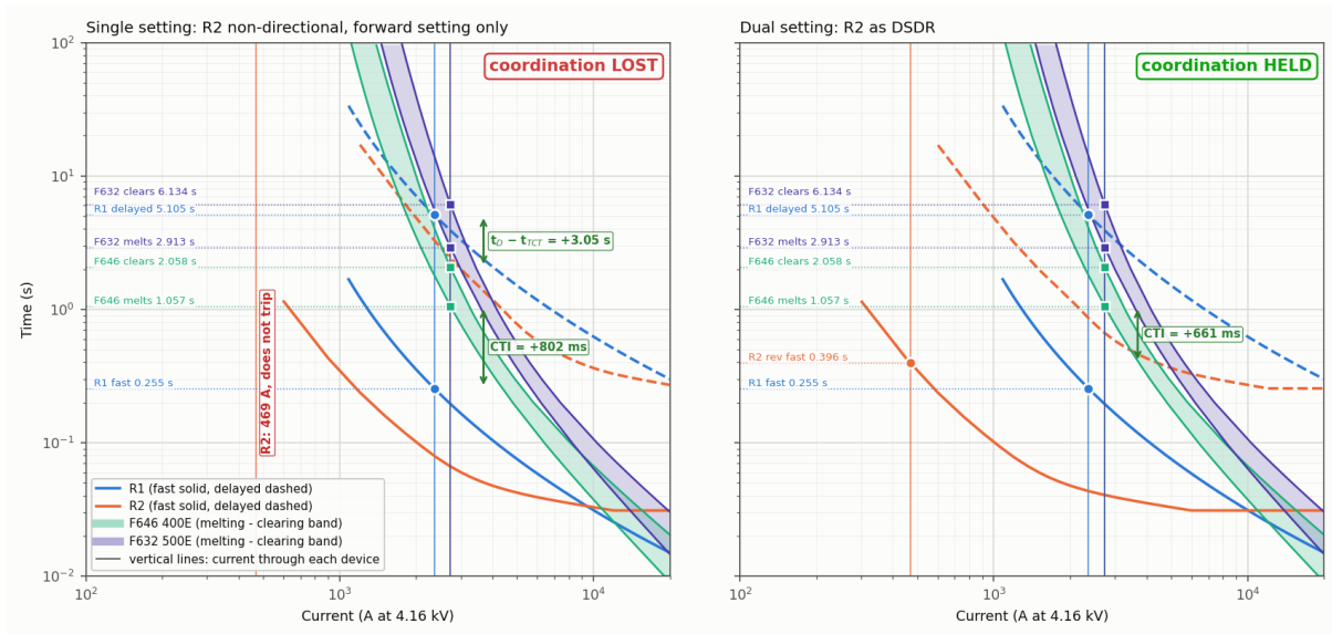
Figure 14: LG fault at 646: the single-setting R2 does not pick up the reverse current (left); the reverse group does (right, CTI = +661 ms).
