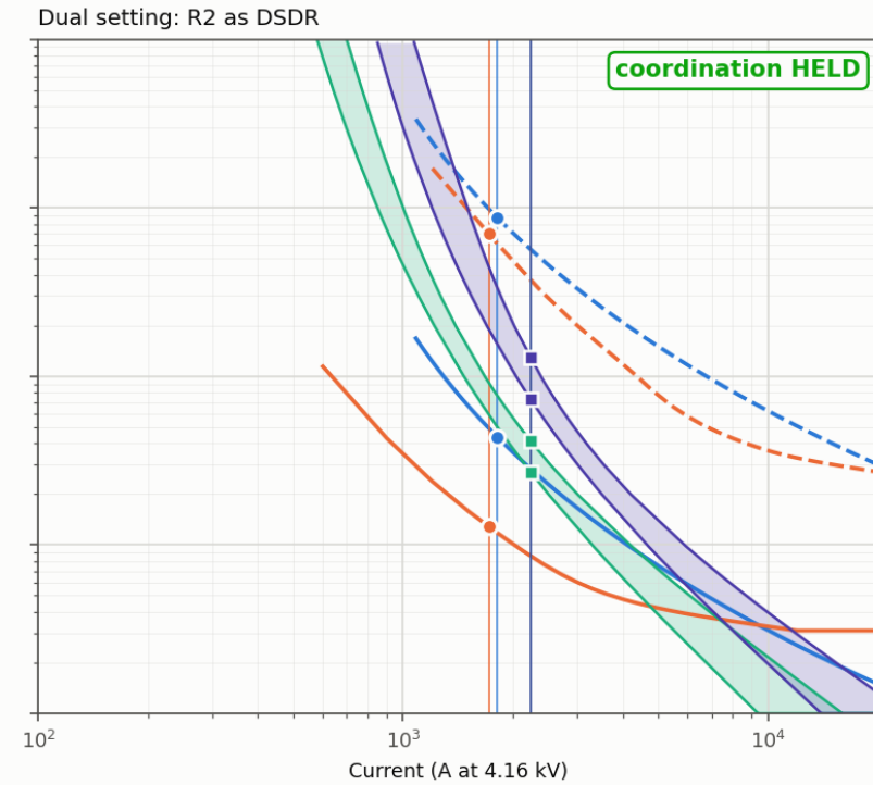
Case 01 - LG fault at 611, Z_f = 0 ohm (bolted), DG 4.05 MVA connected at 692 (Fig. 8)
