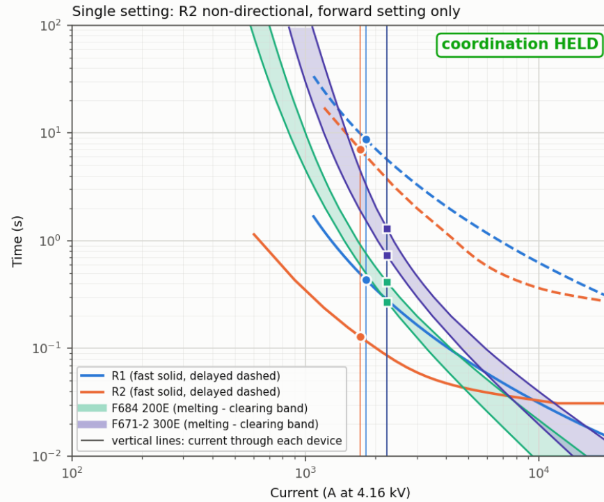
Case 01 - LG fault at 611, Z_f = 0 ohm (bolted), DG 4.05 MVA connected at 692 (Fig. 8)
