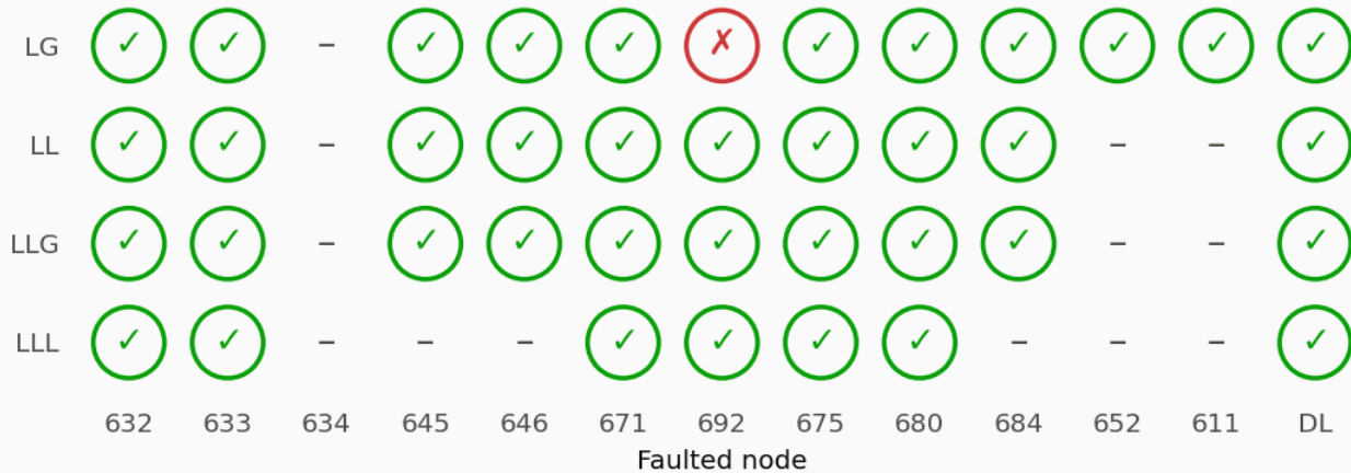
Fig. 17 - coordination with DSDR, DG 4.05 MVA at 692
