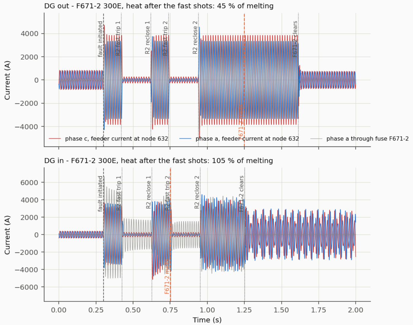
Fig. 10 (replicated) - current at node 632, LL a-c fault at 684 through 0.2 ohm, PowerFactory EMT
