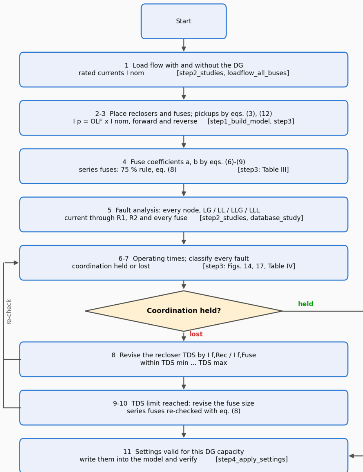
Fig. 5 (redrawn) - the method for recloser-fuse coordination with the DSDR, with the script of each step
