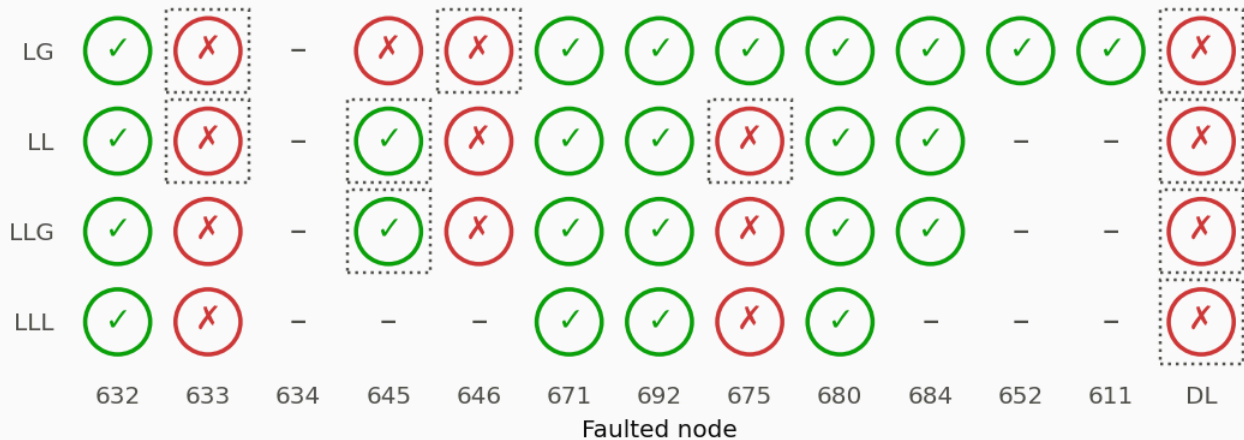
Fig. 14 (replicated) - without DSDR, DG 4.05 MVA at 692
