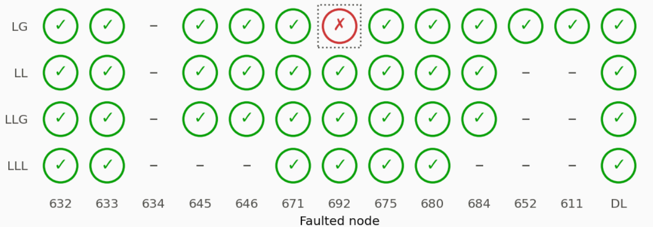
Fig. 17 (replicated) - with DSDR, DG 4.05 MVA at 692
