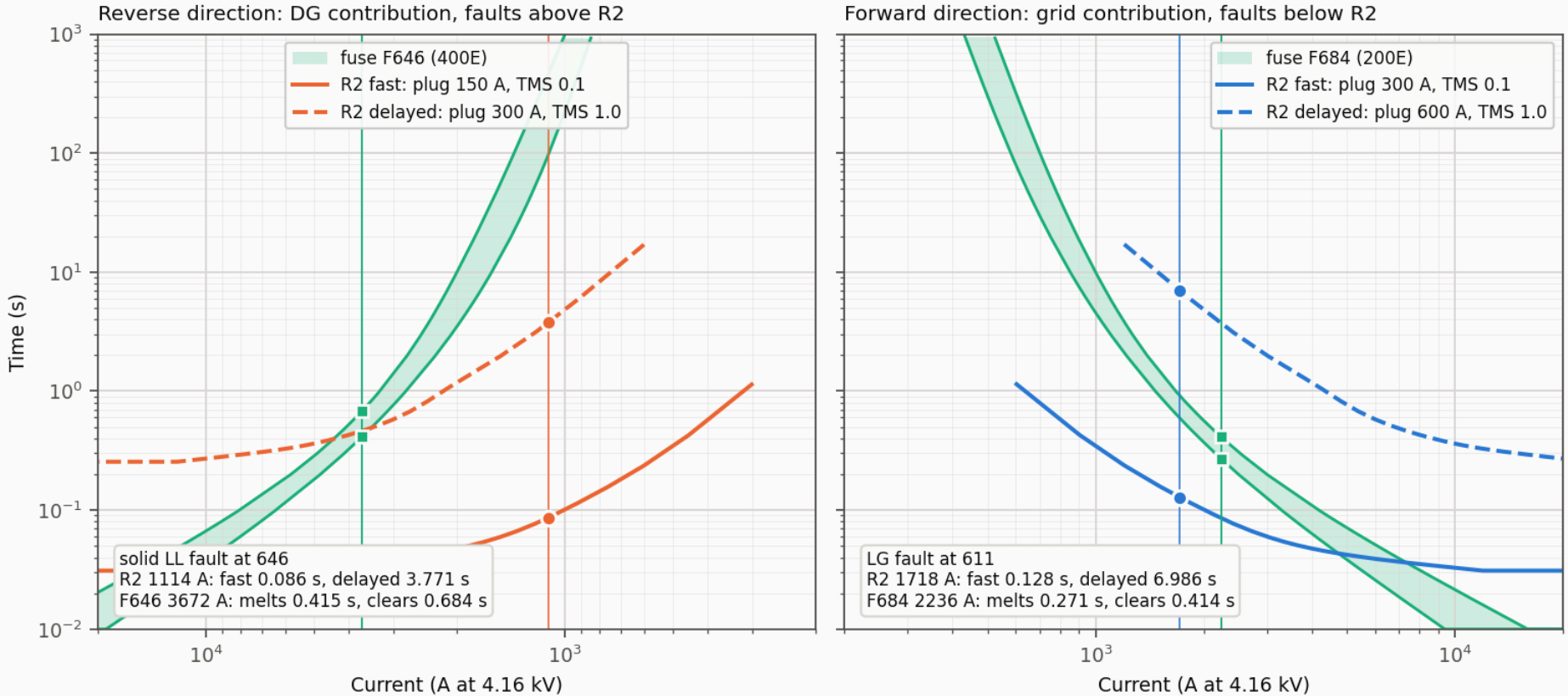
Fig. 3 (replicated) - time-current characteristics of the dual-setting recloser R2: reverse and forward setting
