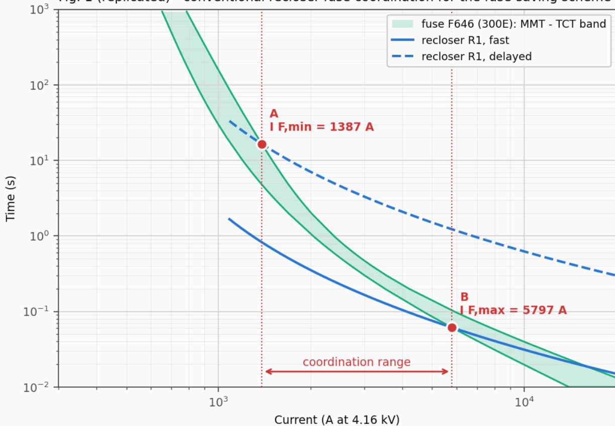
Fig. 1 (replicated) - conventional recloser-fuse coordination for the fuse-saving scheme
