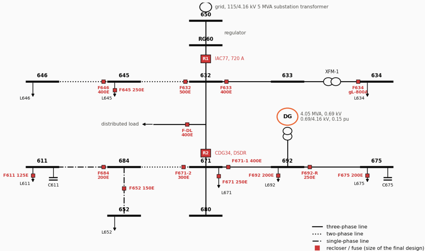
Fig. 6 (redrawn) - IEEE 13-node test feeder with the protective devices of the replication
