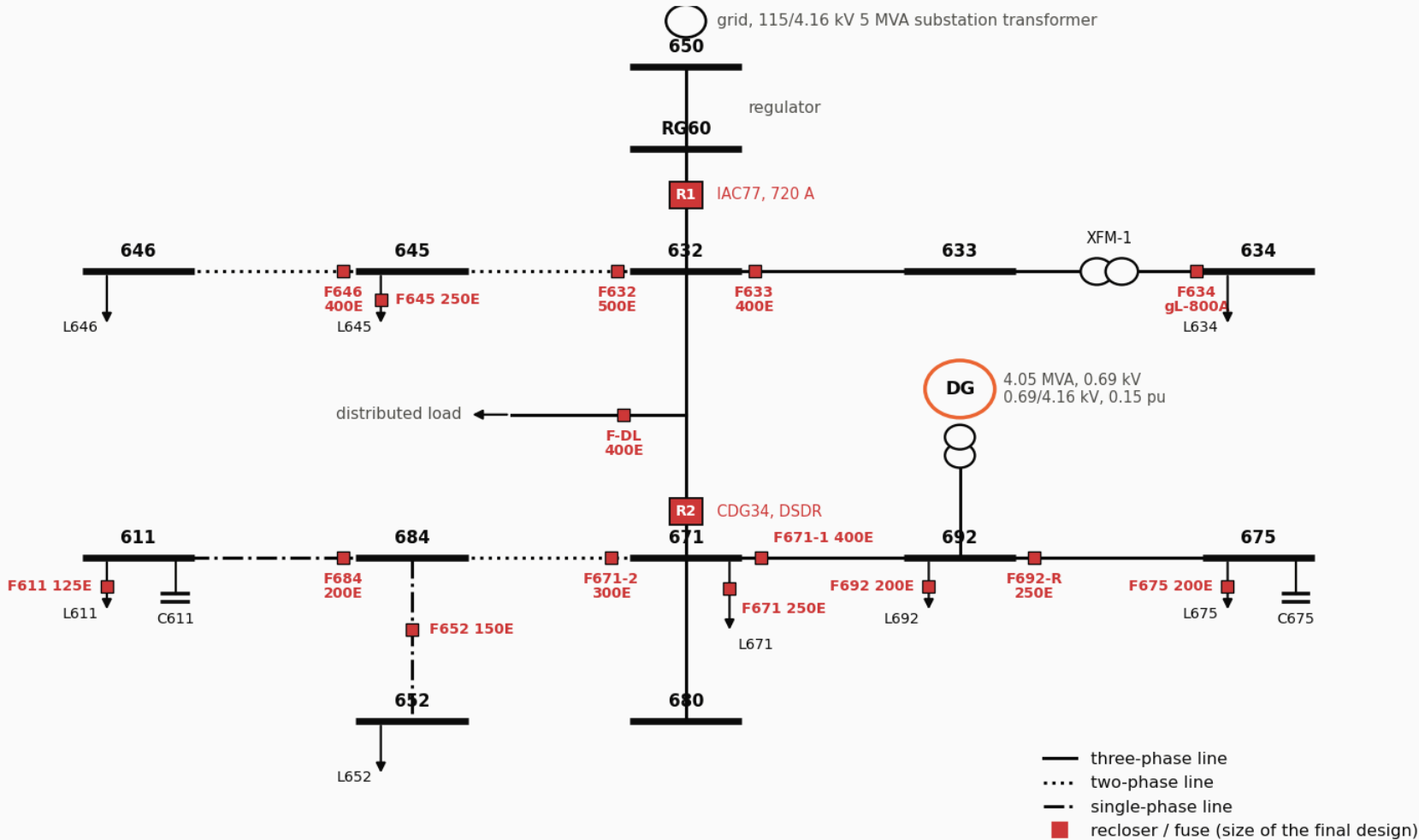
IEEE 13-node test feeder with the protective devices of this study
