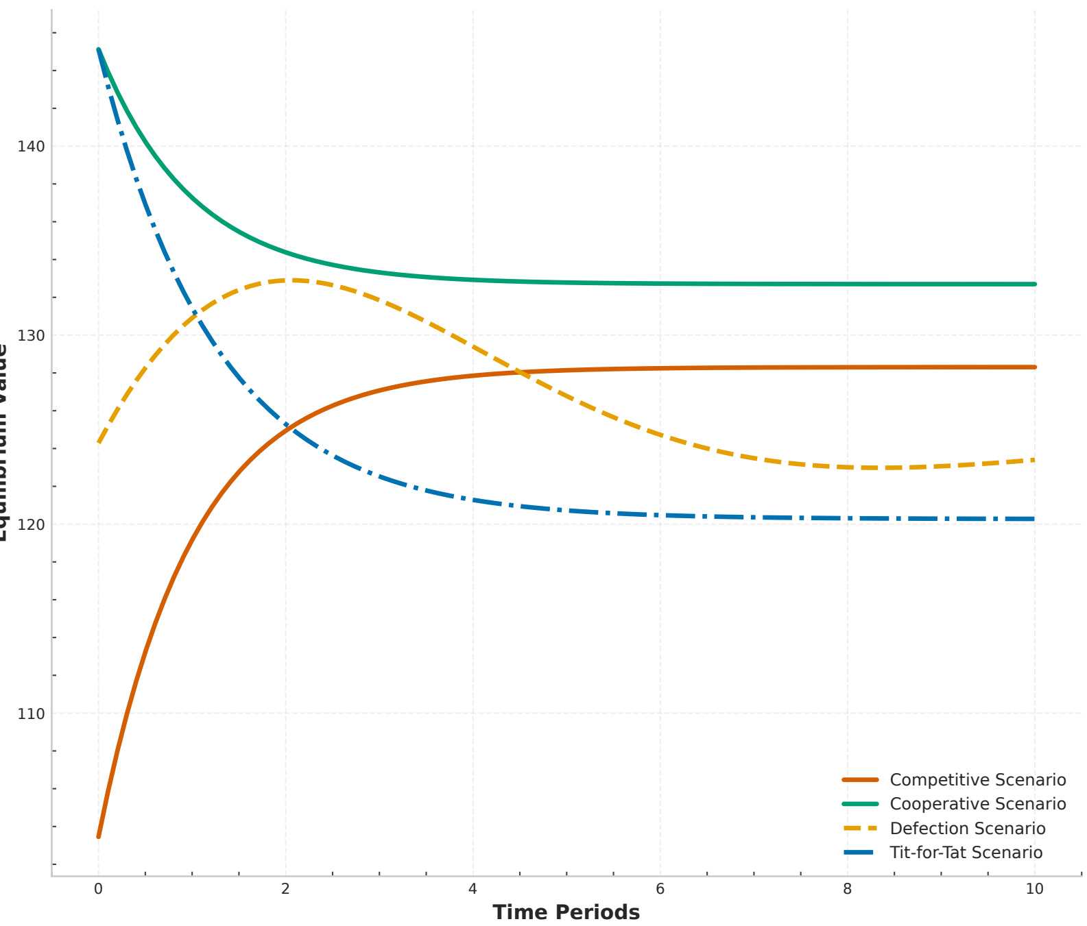
Dynamic Equilibrium Paths (Schematic Trajectories from Calibrated Endpoints)
