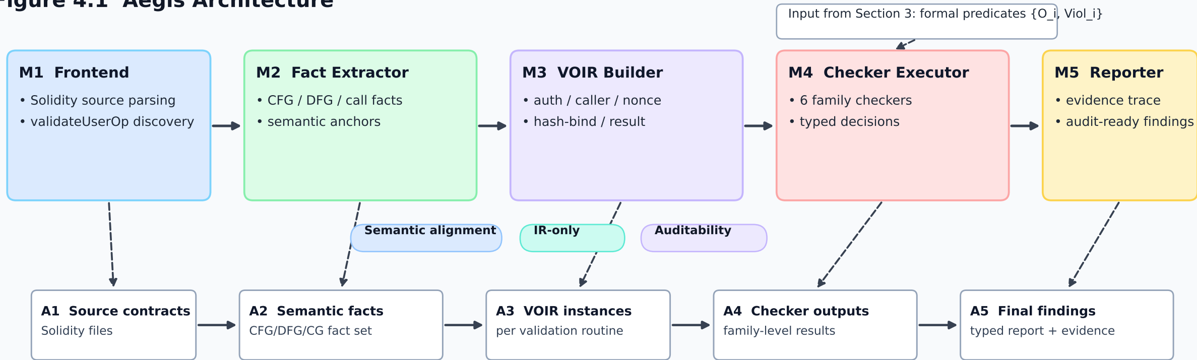
Figure 4.1 Aegis Architecture
