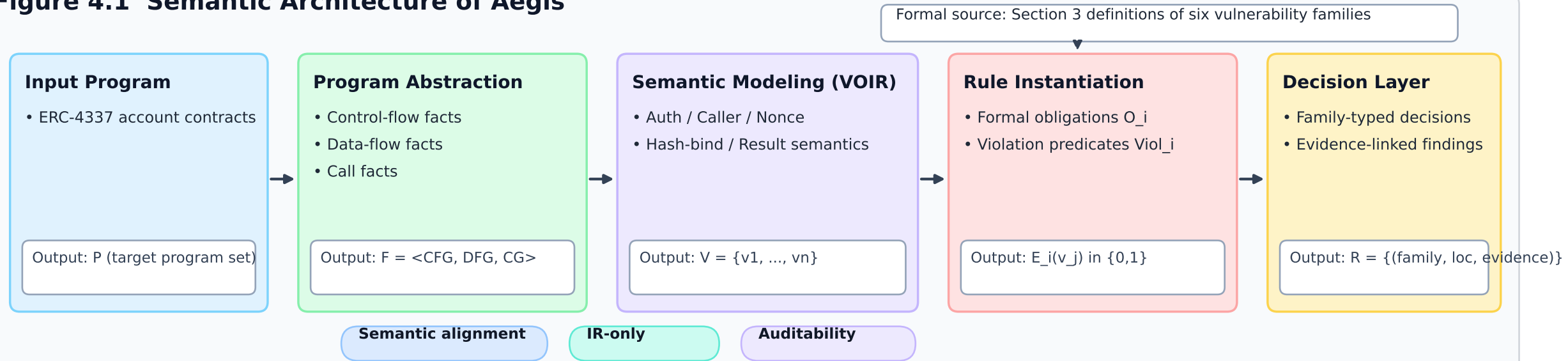
Figure 4.1 Semantic Architecture of Aegis
