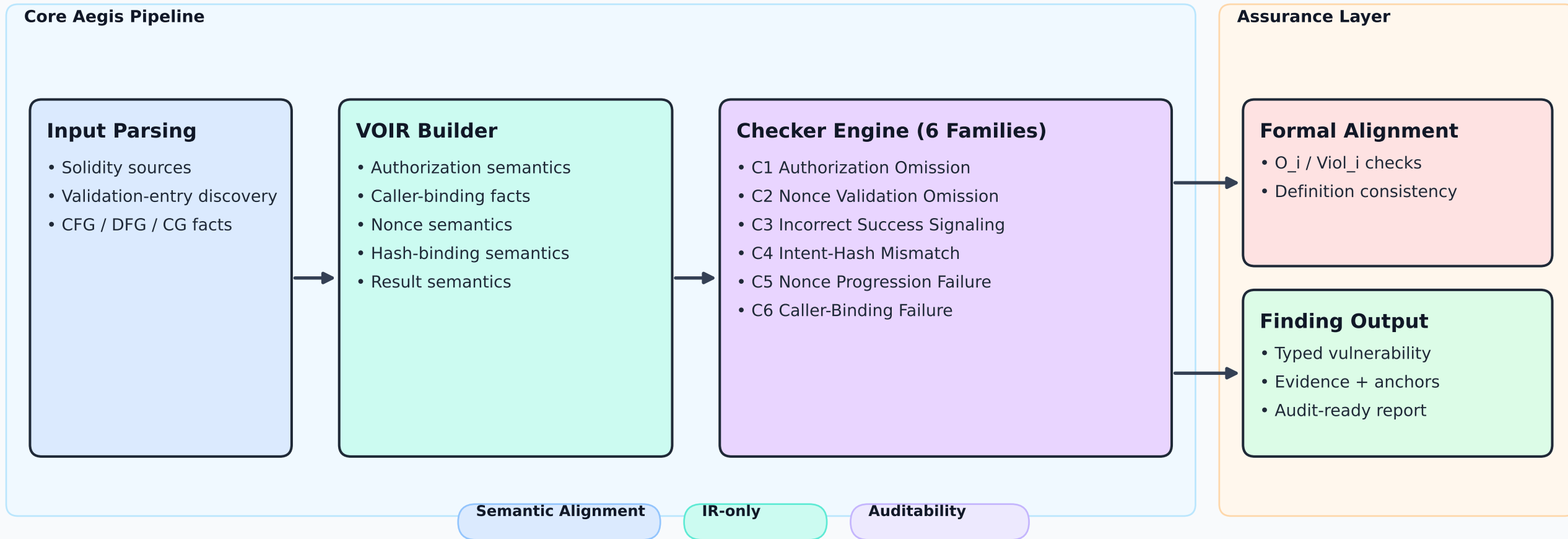
Figure 4.1. Aegis architecture. Source code is transformed into VOIR semantic facts and checked by six formally derived detectors.
