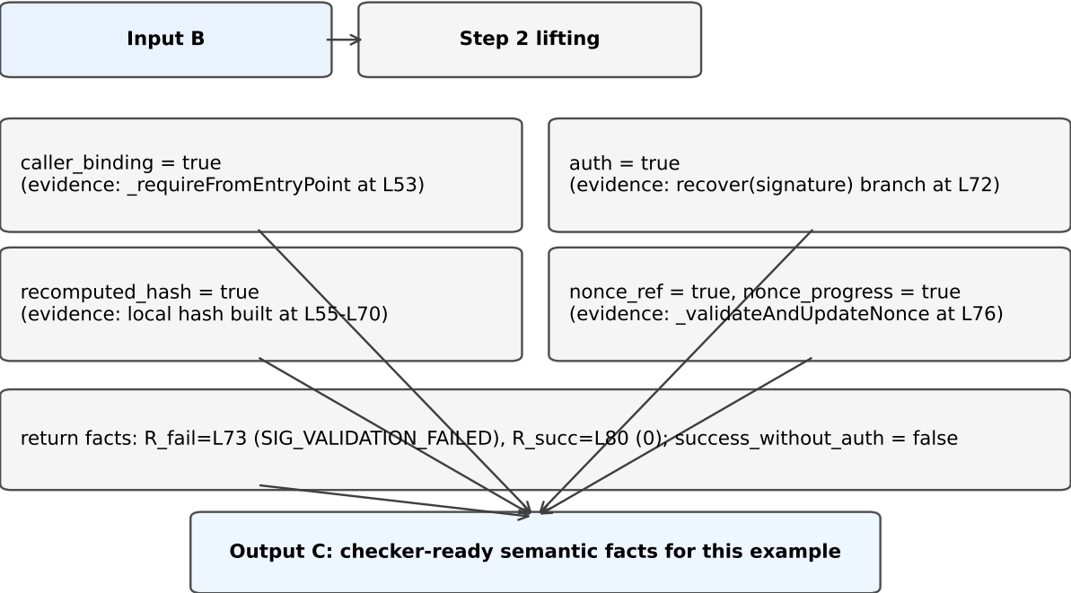
(c) Step 2 Lifted Semantics (Concrete Values)
