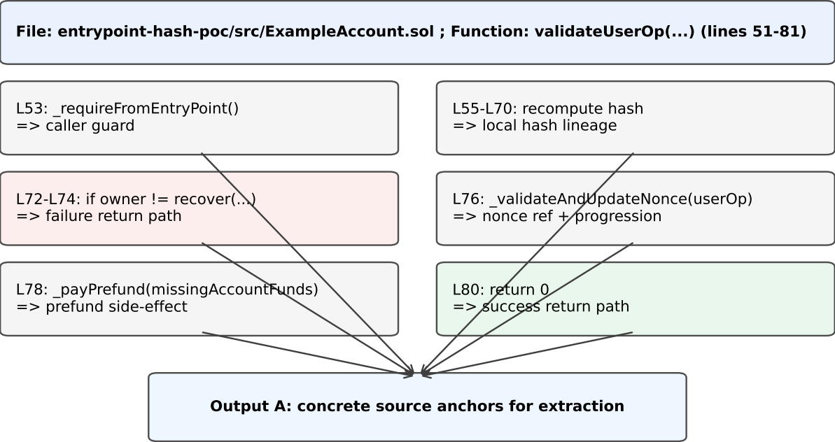
(a) ExampleAccount Source Anchors (Concrete)
