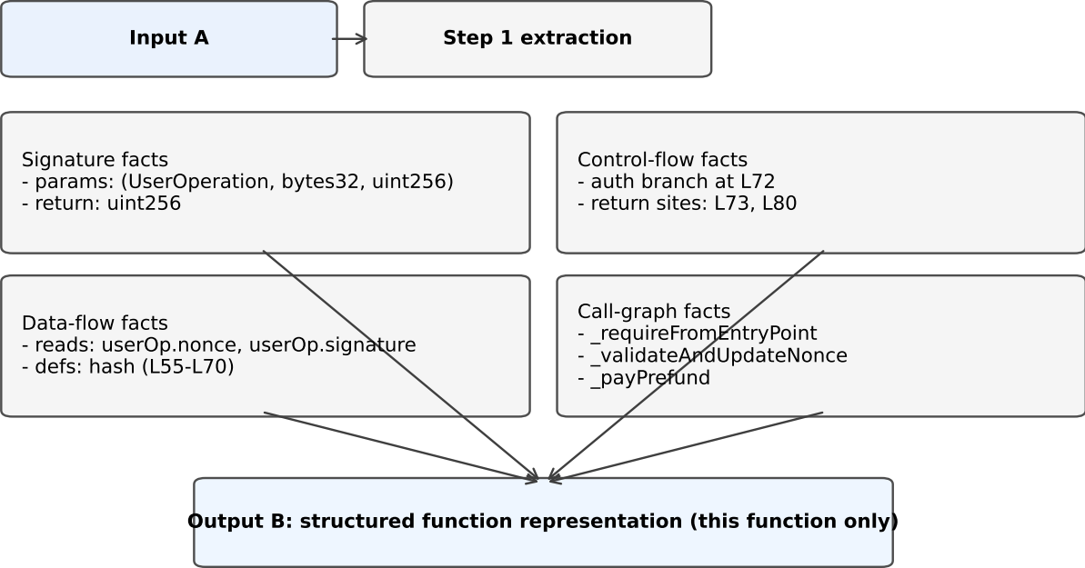
(b) Step 1 Artifacts for This Example (Concrete)
