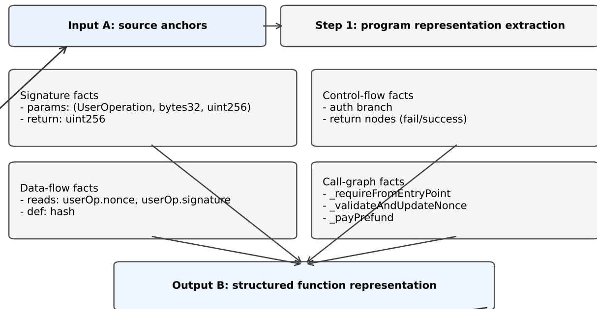
(b) Step 1 Extraction Artifacts
