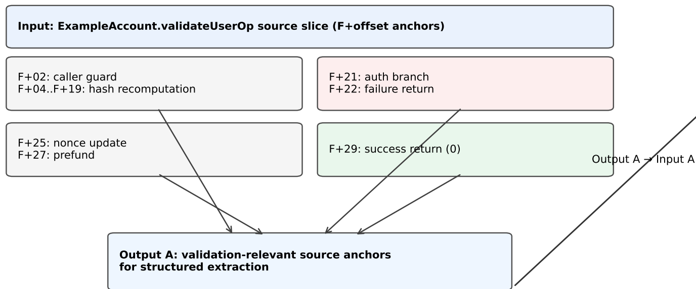
(a) Source Slice with Function-Local Anchors
