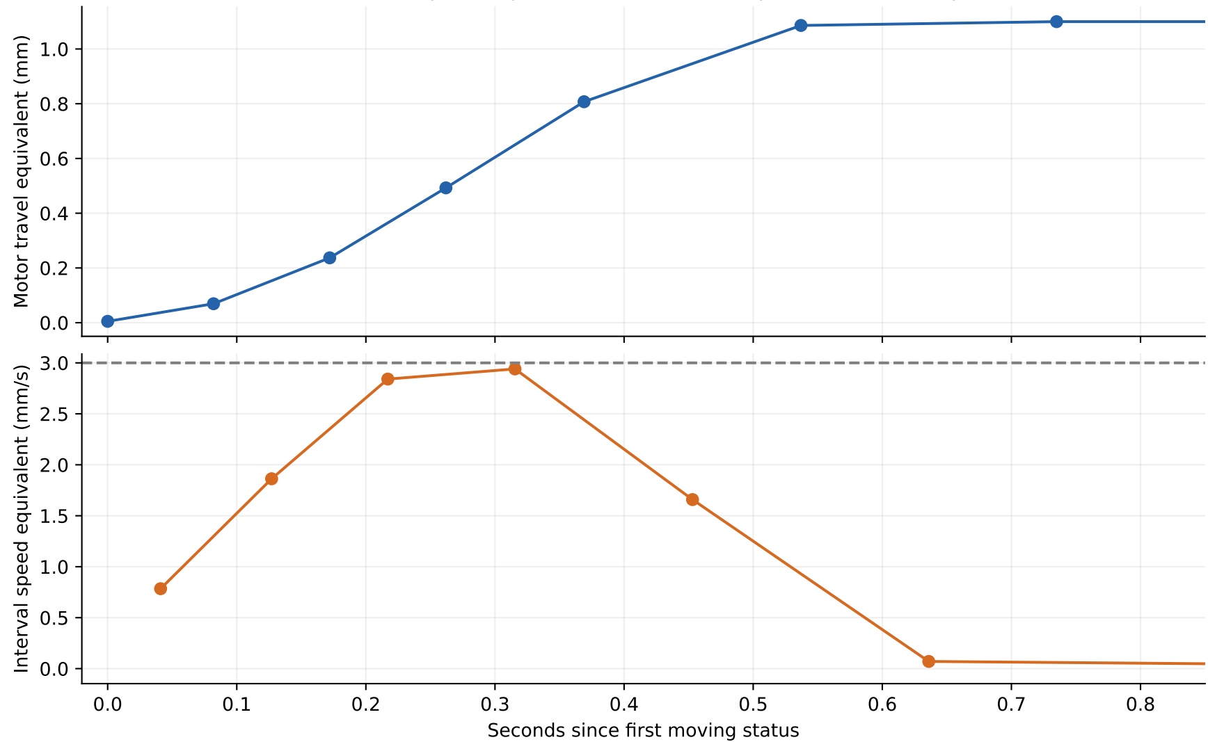
AP +1 mm: reported position and interval speed (3 mm/s request)
