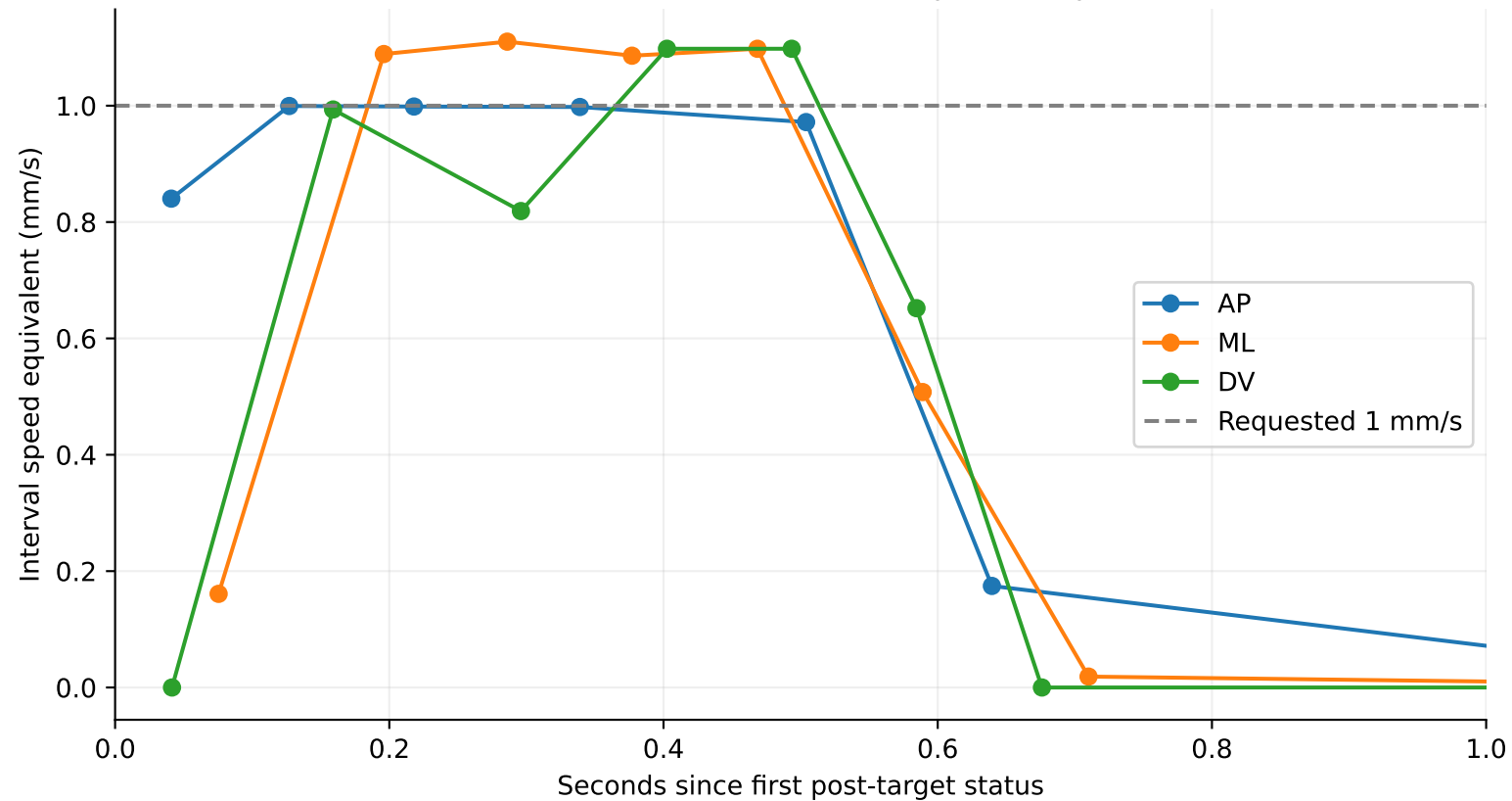
0.5 mm moves at the same requested speed
