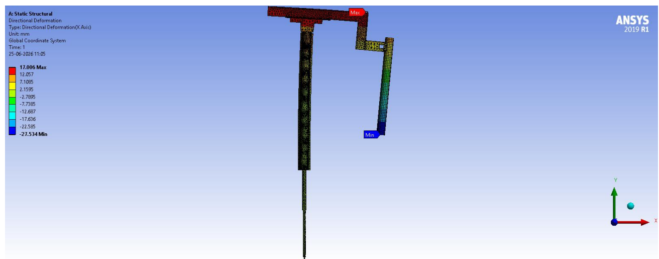
57. X-axis Deformation
