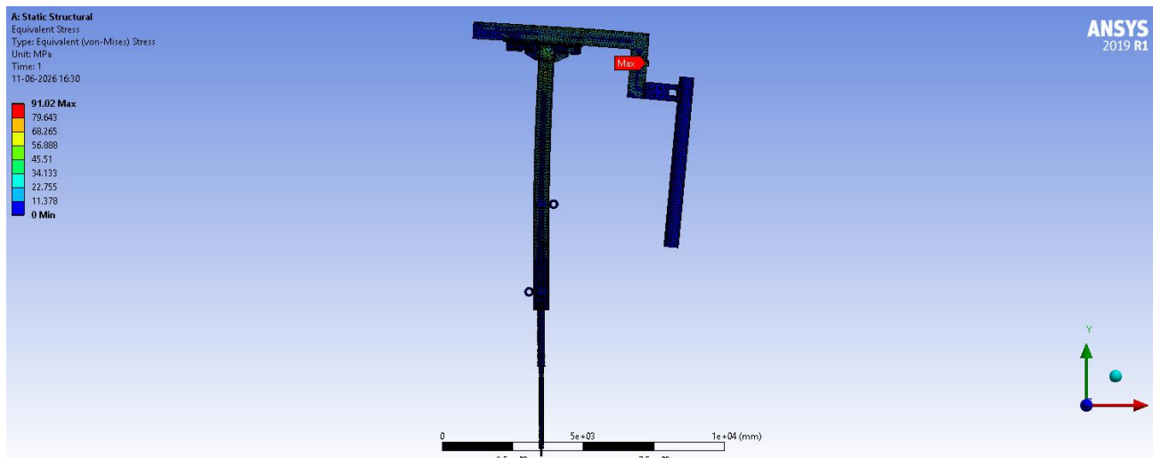
33. Equivalent Stress
