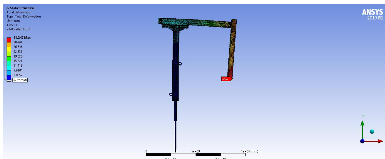
14. Total Deformation
