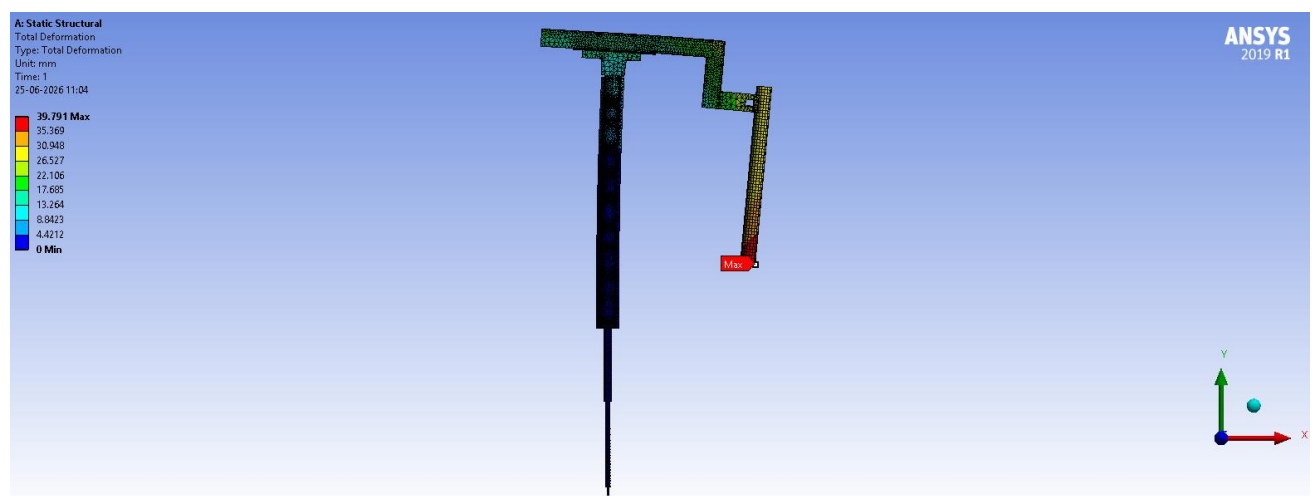
56. Total Deformation
