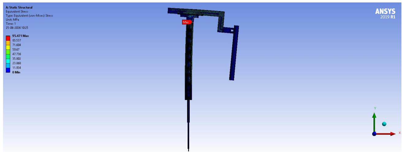
55. Equivalent Stress
