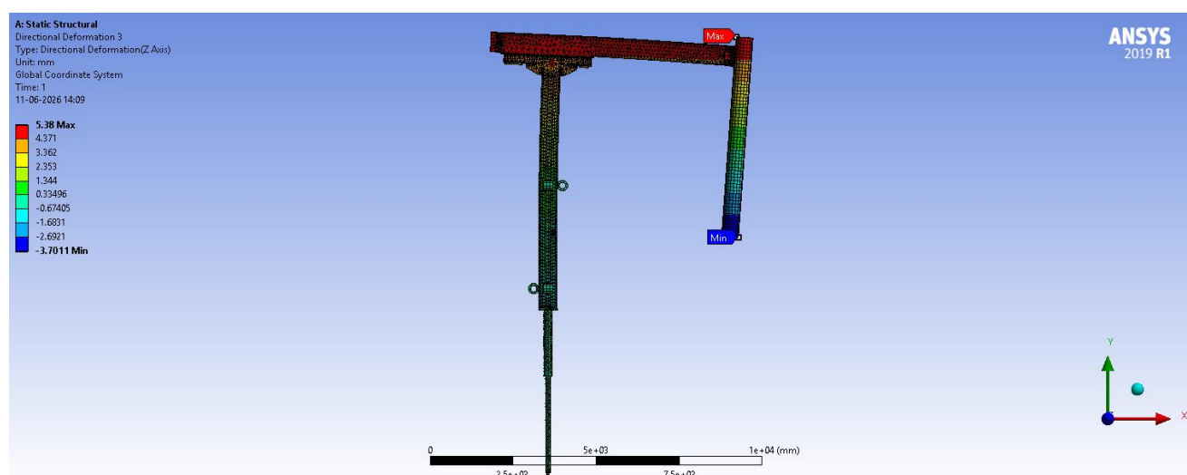
26. Z-axis Deformation
