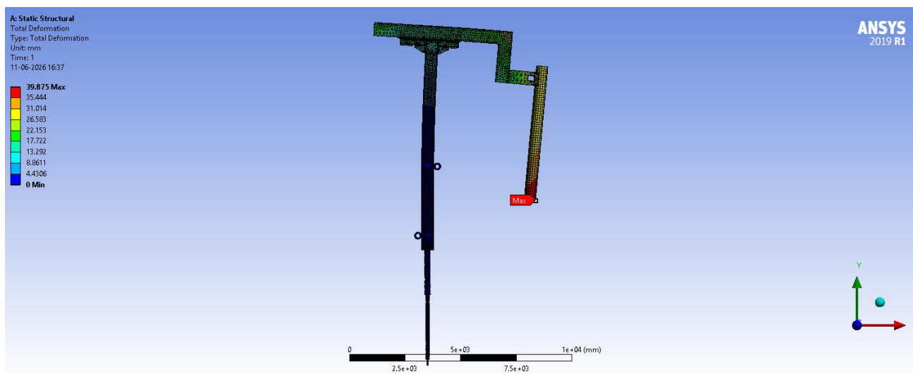
34. Total Deformation
