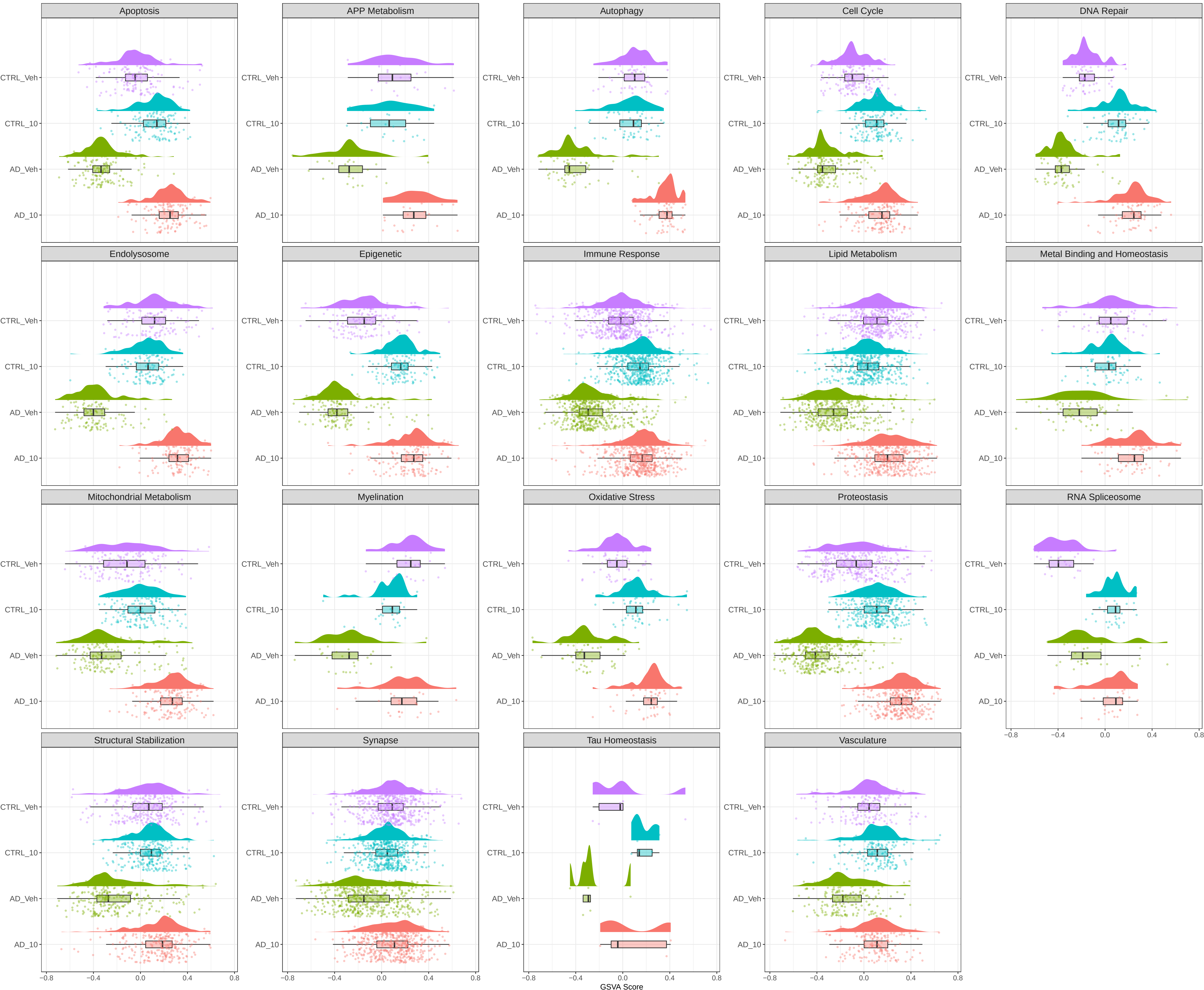
GSVA Distribution per Biomain (Raincloud Plot)
