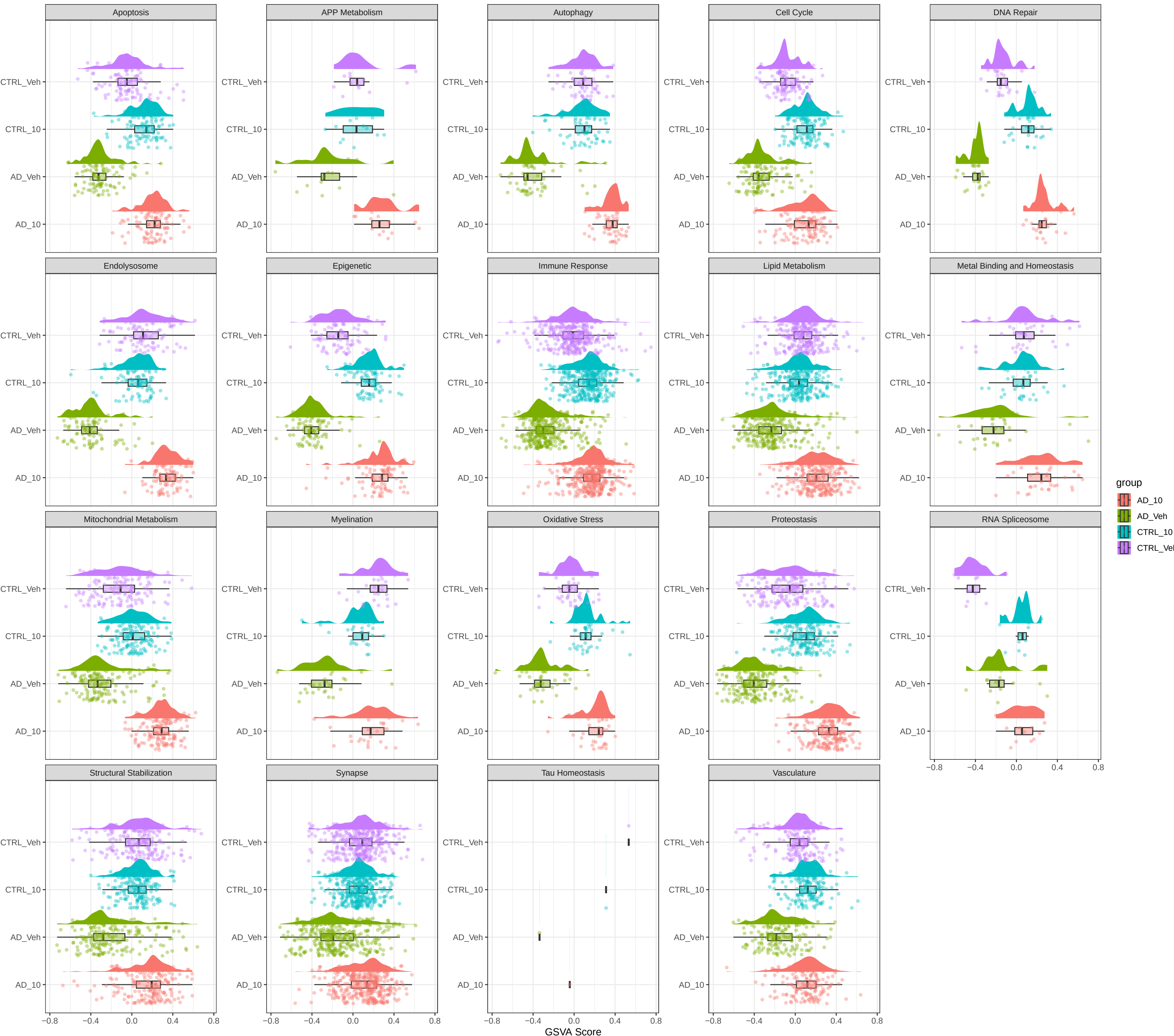
GSVA Distribution per Biodomain (Raincloud Plot)
