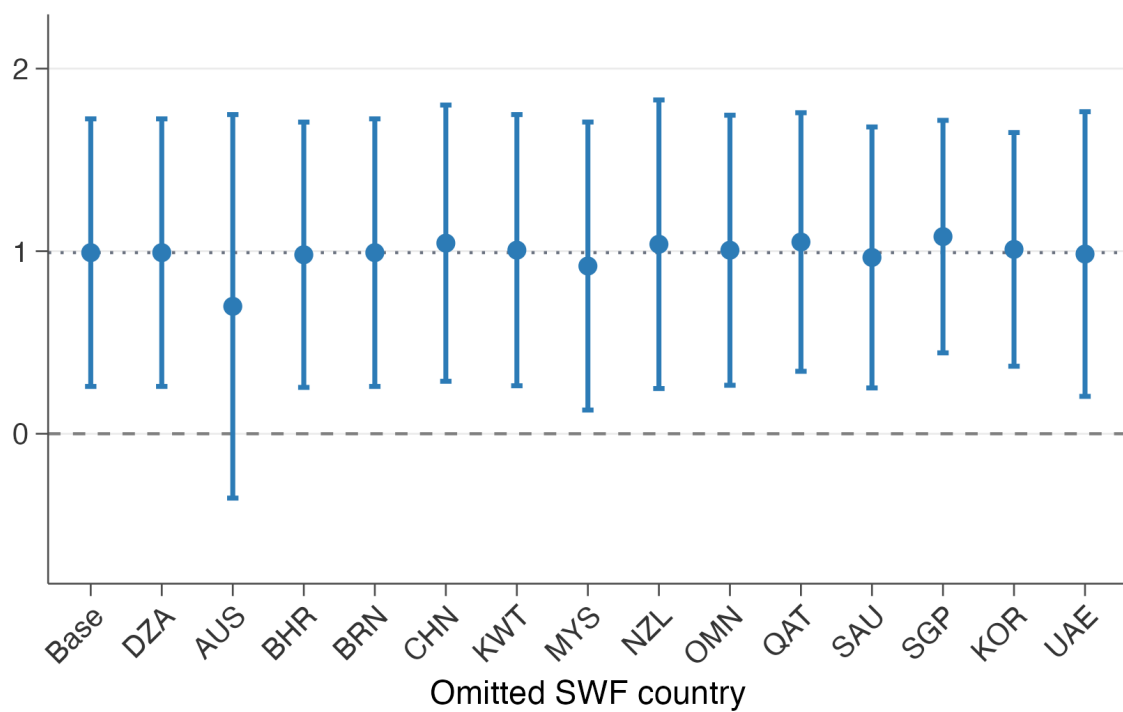
Figure 12: Leave-One-SWF-Country-Out: Deal Count
