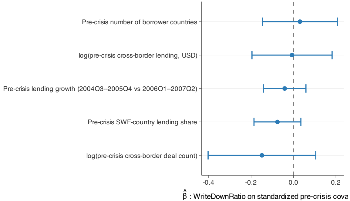
Figure 10: Bank Pre-Crisis Balance: WriteDownRatio on Standardized Covariates Notes: Cross-sectional OLS of the bank-level WriteDownRatio on five standardized pre-crisis covariates (N=18 banks). Pre-crisis covariates aggregate the bank–country–quarter panel over 2004Q3–2007Q2: total cross-border lending (USD), deal count, number of borrower countries, share of total lending to SWF home countries, and a pre-crisis lending growth measure defined as the log of total lending in 2006Q1–2007Q2 relative to 2004Q3–2005Q4. Each covariate is standardized to mean zero and unit standard deviation. Error bars: 95% confidence intervals from OLS standard errors. Coefficients near zero indicate balance; any residual level differences are absorbed by the Bank×Country and WD × Pre-share × Post controls in the main specification.
