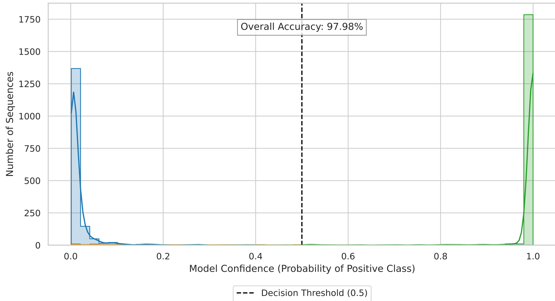
Prediction Confidence Distribution - HMB-Net (Atlas_h_m1A)
