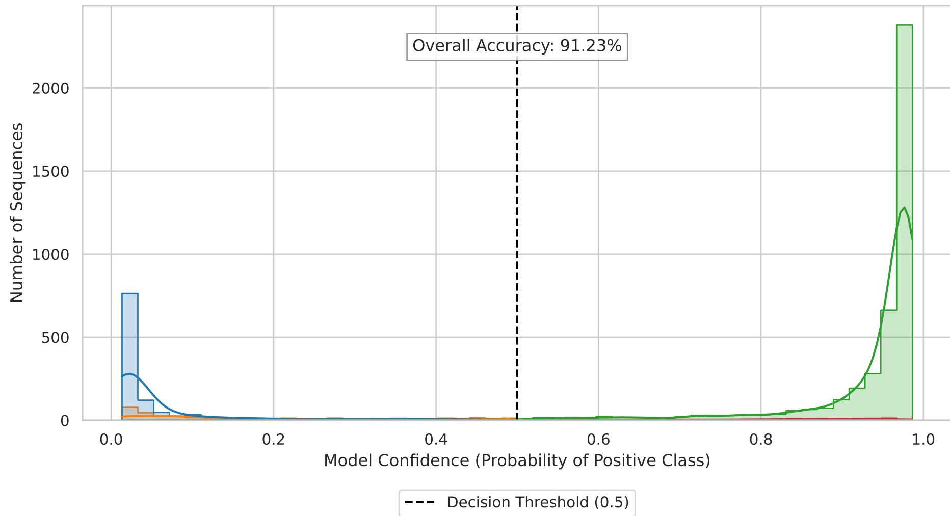
Prediction Confidence Distribution - HMB-Net (Atlas_h_m5C)
