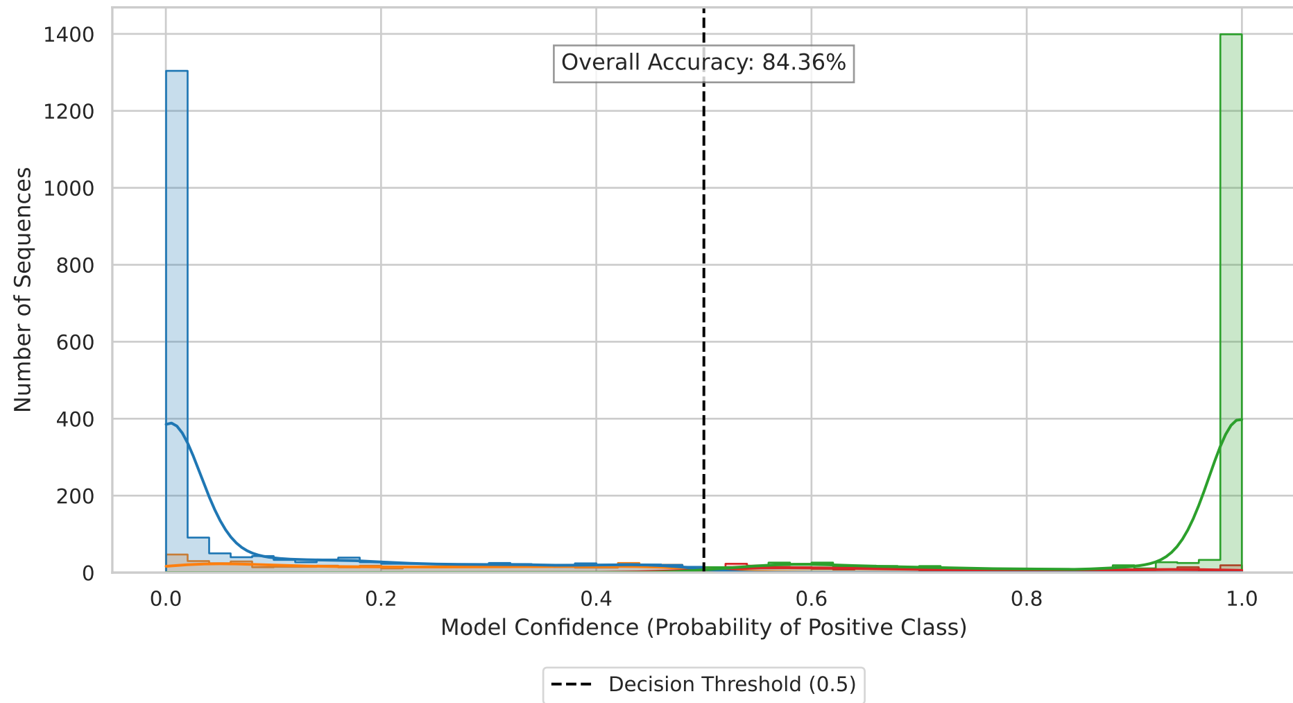
Prediction Confidence Distribution - HMB-Net (Atlas_m_m1A)
